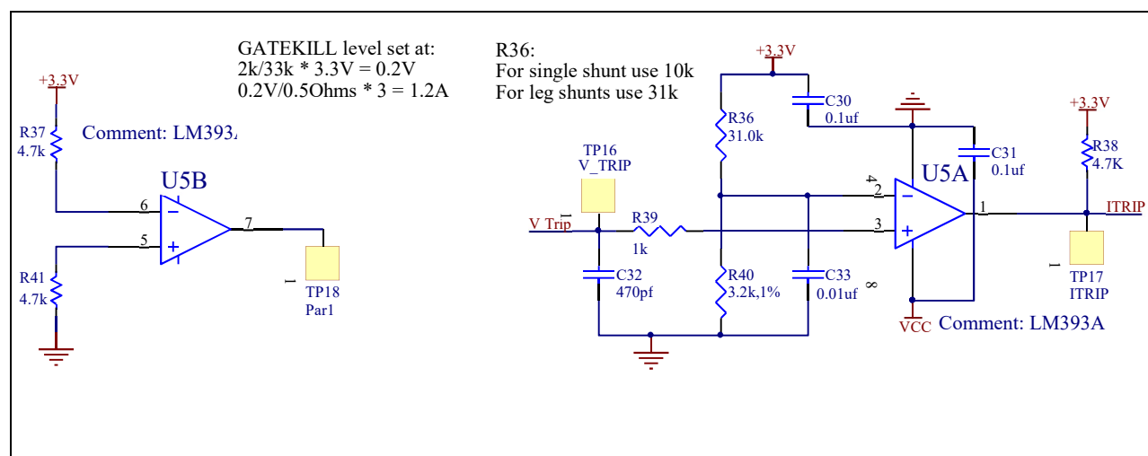
Figure 13 Over current protection circuit on the EVAL-M1-36-44A evaluation board
