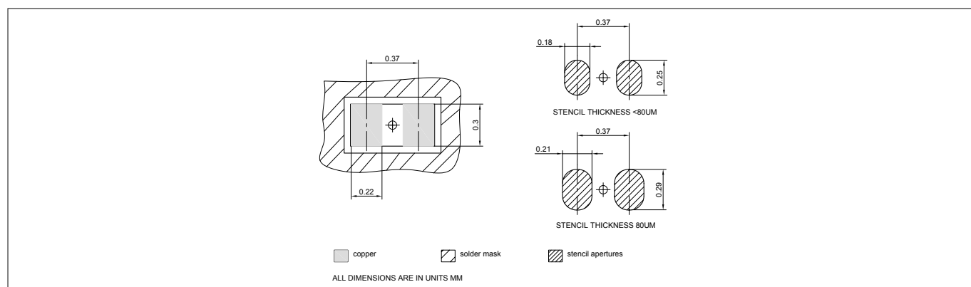
Figure 13 WLL-2-3 footprint (dimension in mm), recommendation for Printed Circuit Board Assembly see [2]
