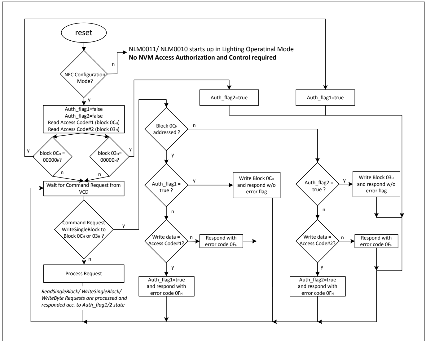
Figure 8 Access Authorization Flow Chart
