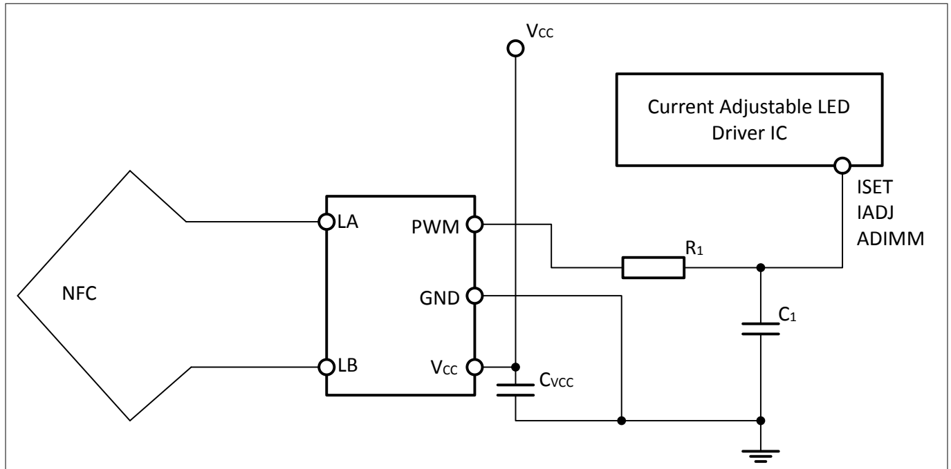
Figure 1 NLM0011 Application View
