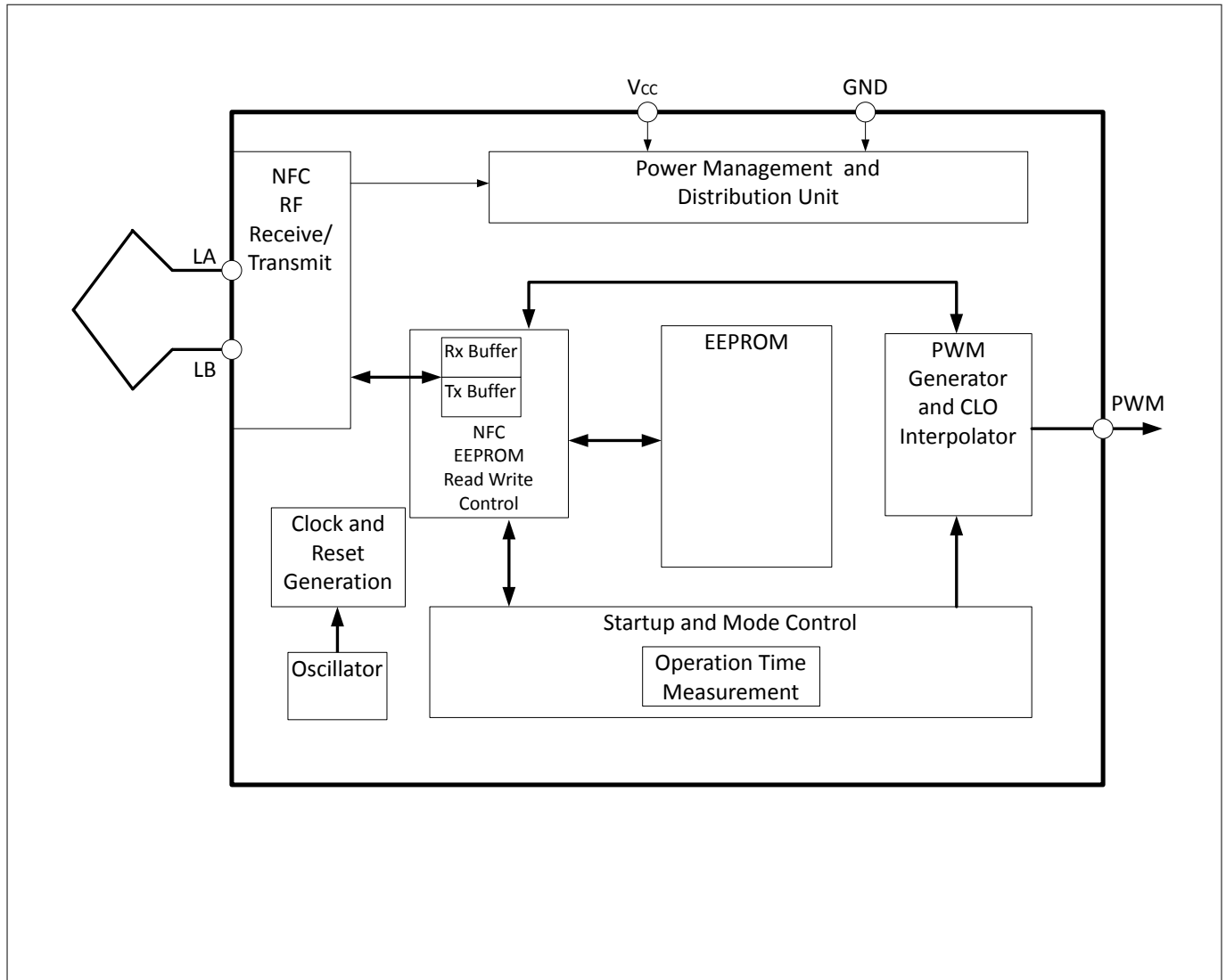
Figure 3 Block Diagram
