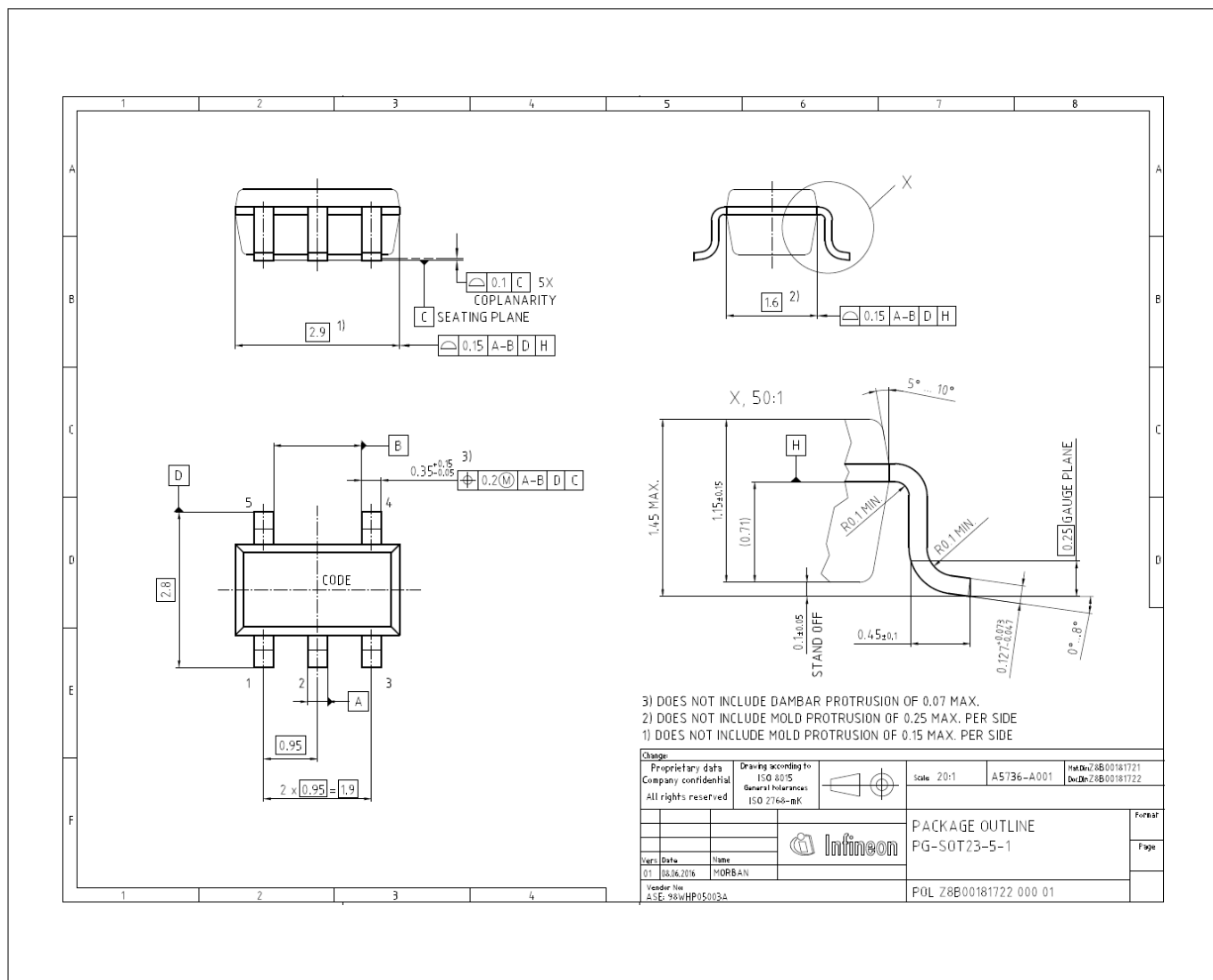
Figure 15 Package Outline PG-SOT23-5-1
