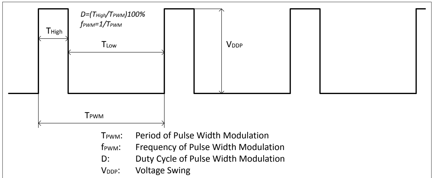
Figure 14 PWM Output Characteristics
