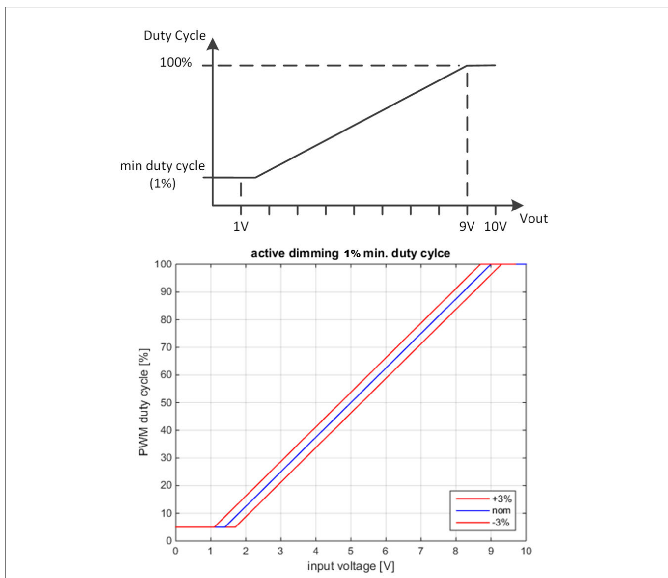
Figure 4 Dimming Characteristic
