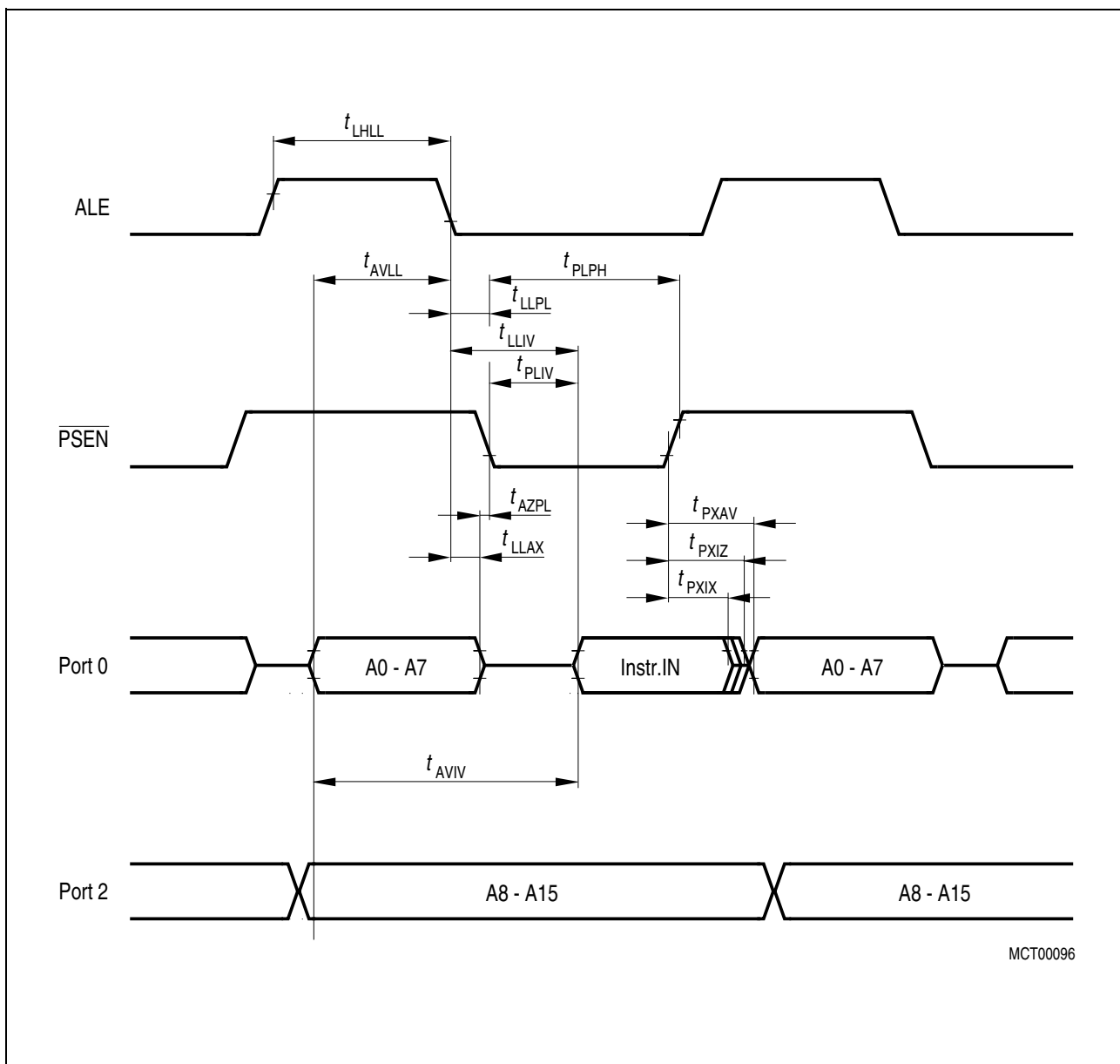
Figure 30 Program Memory Read Cycle
