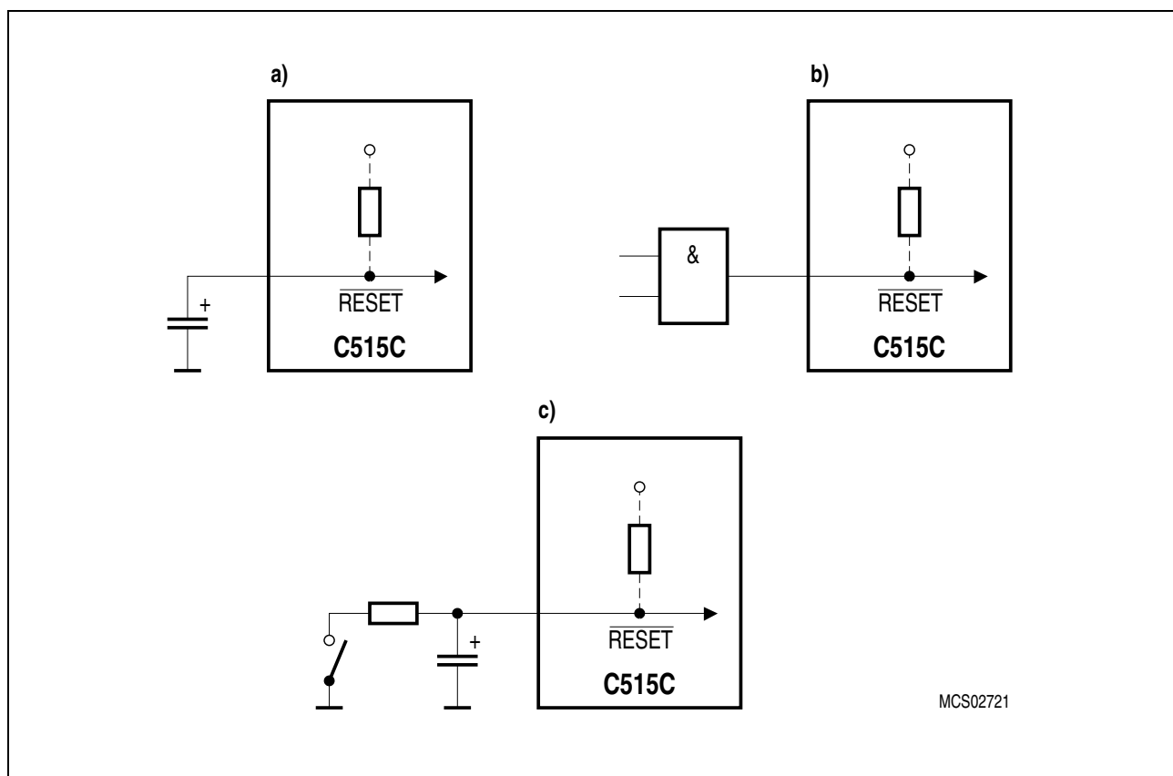
Figure 6 Reset Circuitries
