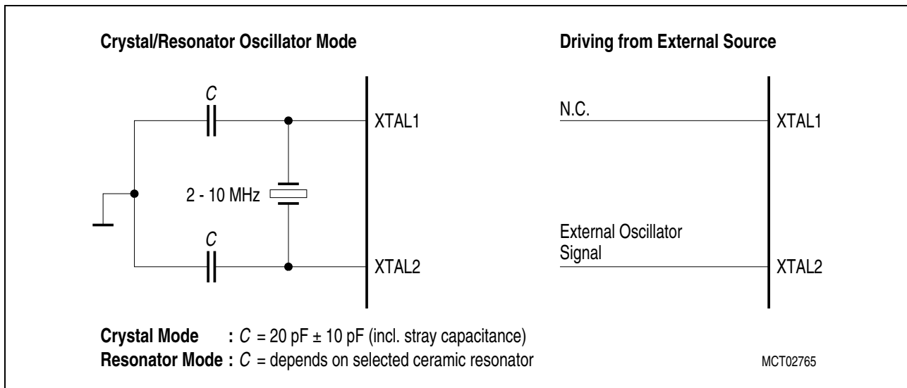
Figure 7 Recommended Oscillator Circuitries
