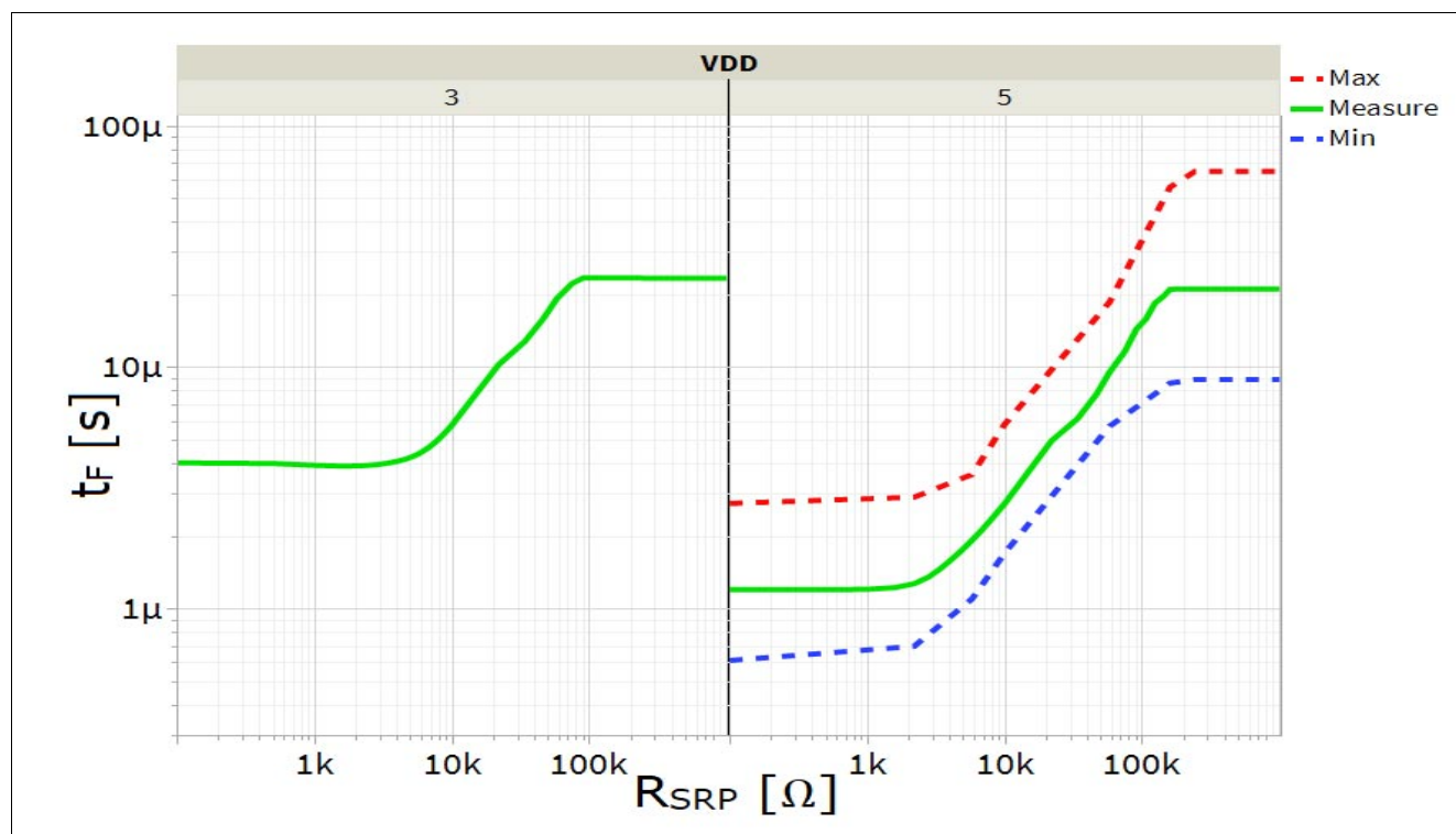
Figure 23 Typical t_F vs. R_{SRP} @ V_{IN} = 5V ; V_{DD} = 3V, 5V ; V_{BAT} = 28V ; R_L = 4.7\Omega ; T_J = [-40 \dots 150^\circ C]
