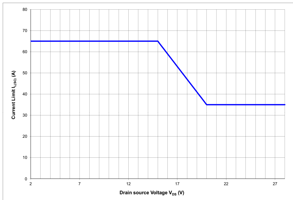
Figure 18 Current Limitation (typical behavior)
