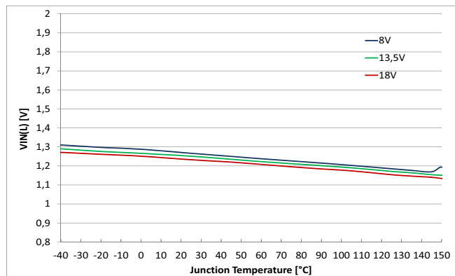
Figure 49 Input Voltage Threshold V_{IN(L)} = f(T_J; V_S)
