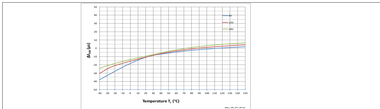
Figure 39 Turn ON / OFF matching \Delta t_{SW} = f(T_j; V_{GS}) , R_L = 2 \Omega
