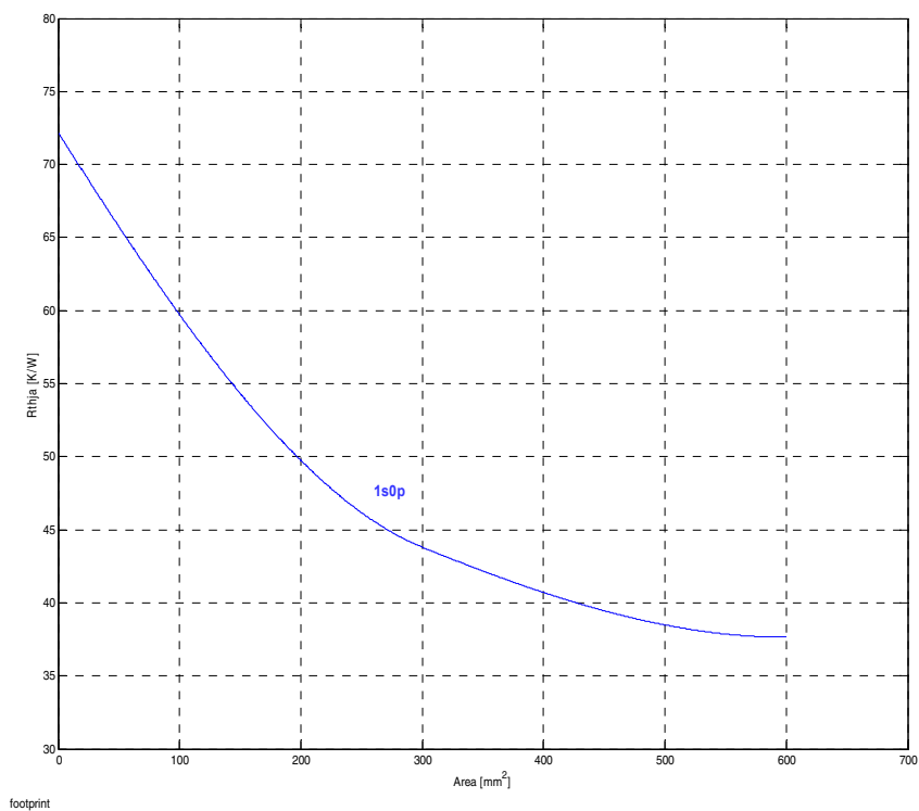
Figure 7 Typical Thermal Resistance. PCB set up 1s0p
