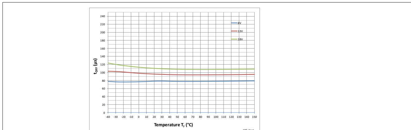
Figure 38 Turn OFF t_{OFF} = f(T_j; V_{GS}) , R_L = 2 \Omega
