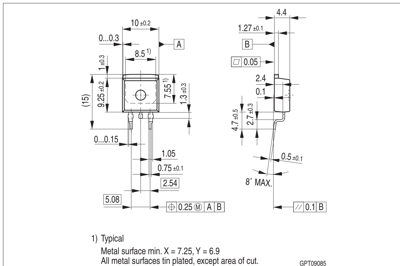
Figure 16 PG-TO263-3-2 (Plastic Dual Small Outline Package - D²PAK)
