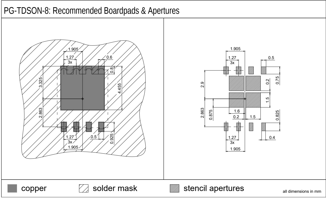
Figure 3 Outline Boardpads (TDSON-8), dimensions in mm
