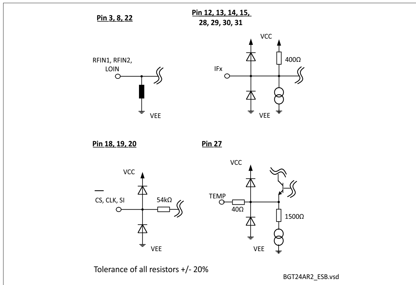
Figure 7 Equivalent Circuit Diagram of MMIC Interfaces
