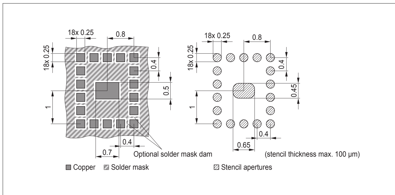
Figure 5: Land Pattern and Stencil Mask
