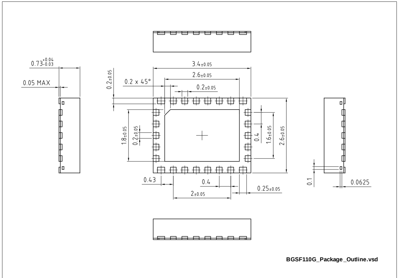
Figure 3 Package Outline
