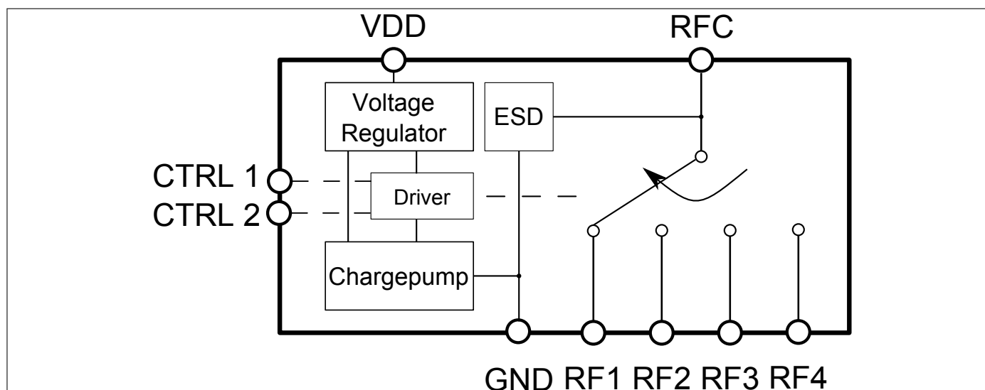
Figure 1: BGSA14GN10 block diagram
