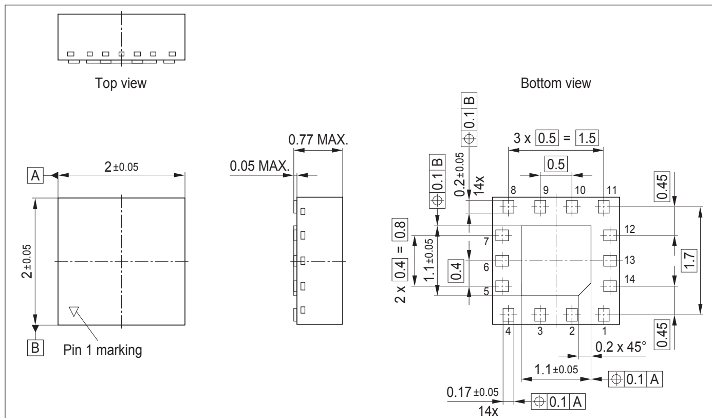
Figure 10: Package outline
