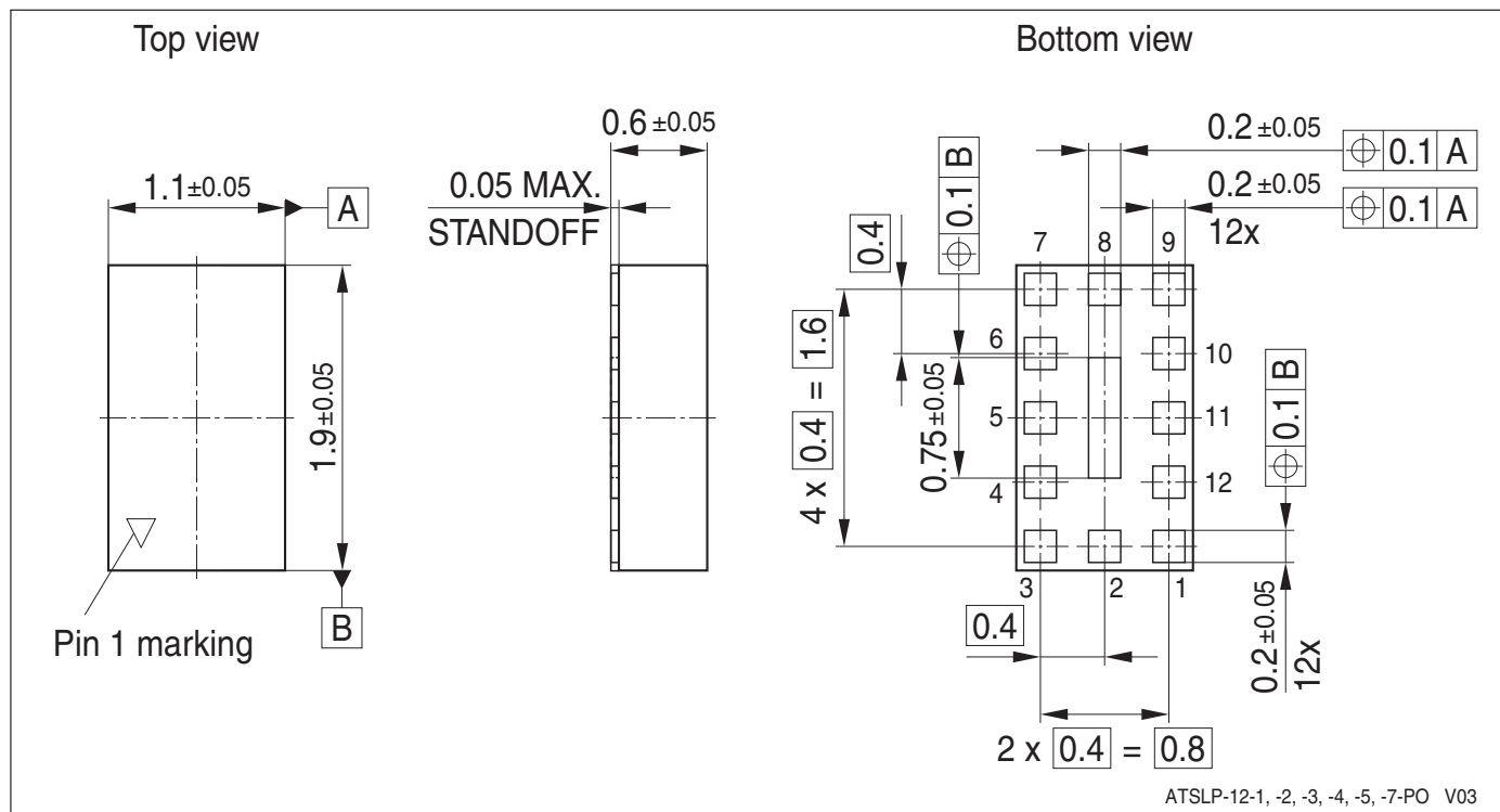
Figure 11: ATSLP-12-4 Package Outline (top, side and bottom views)
