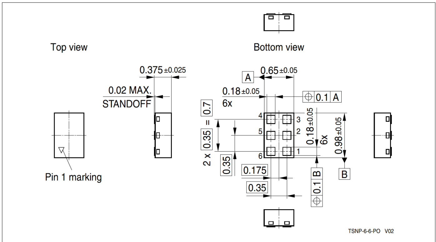
Figure 3: Package Outline
