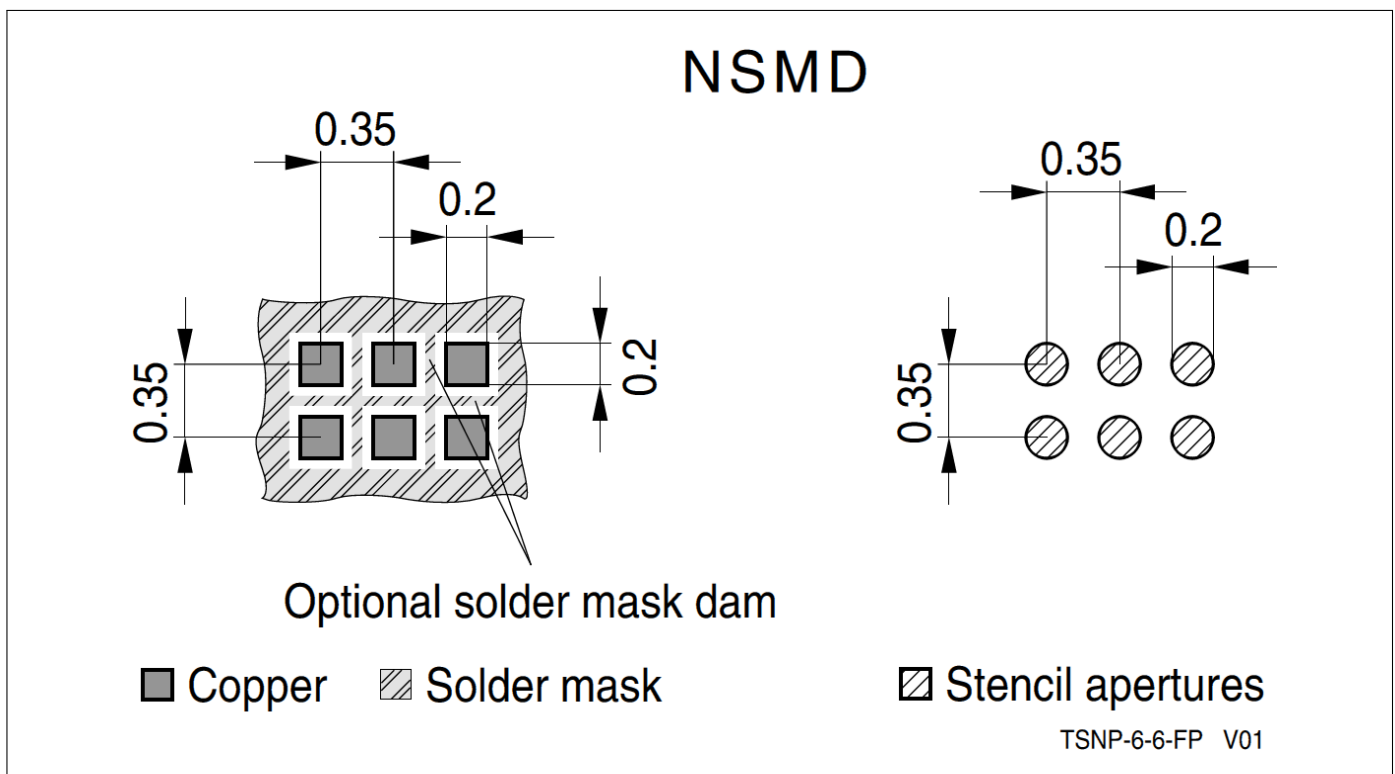
Figure 4: Footprint
