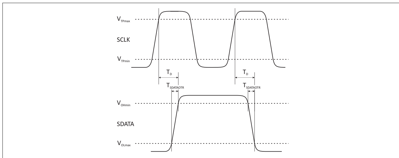
Figure 5: Bus active data transmission timing specification
