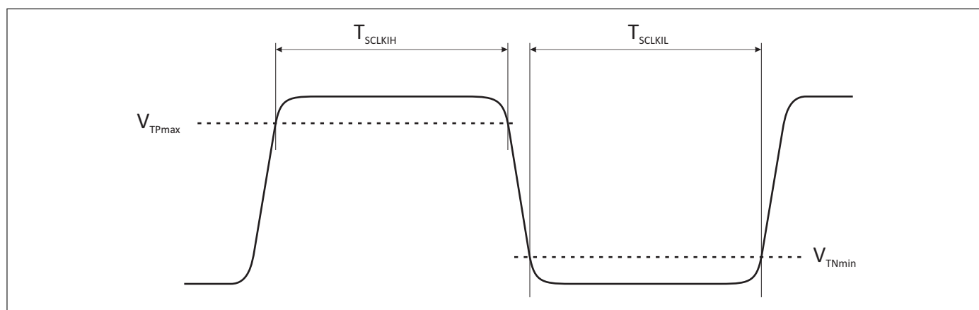
Figure 2: Received clock signal constraints
