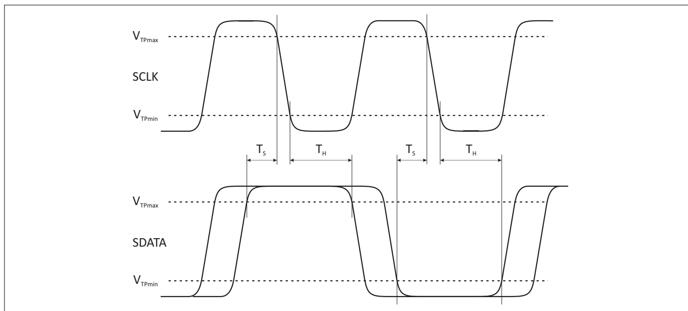
Figure 3: Bus active data receiver timing requirements
