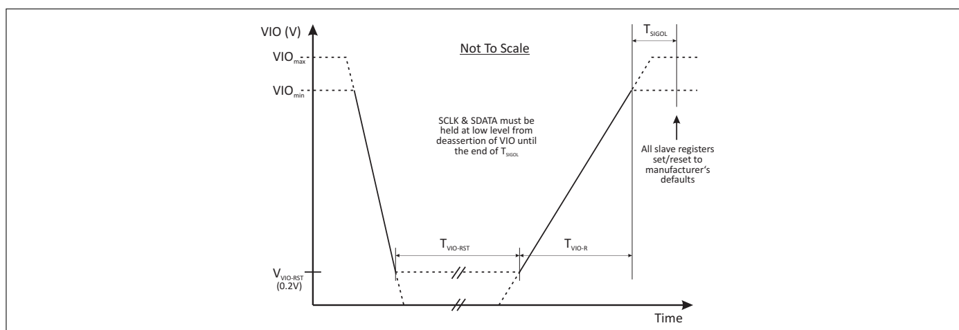
Figure 6: Requirements for VIO-initiated reset
