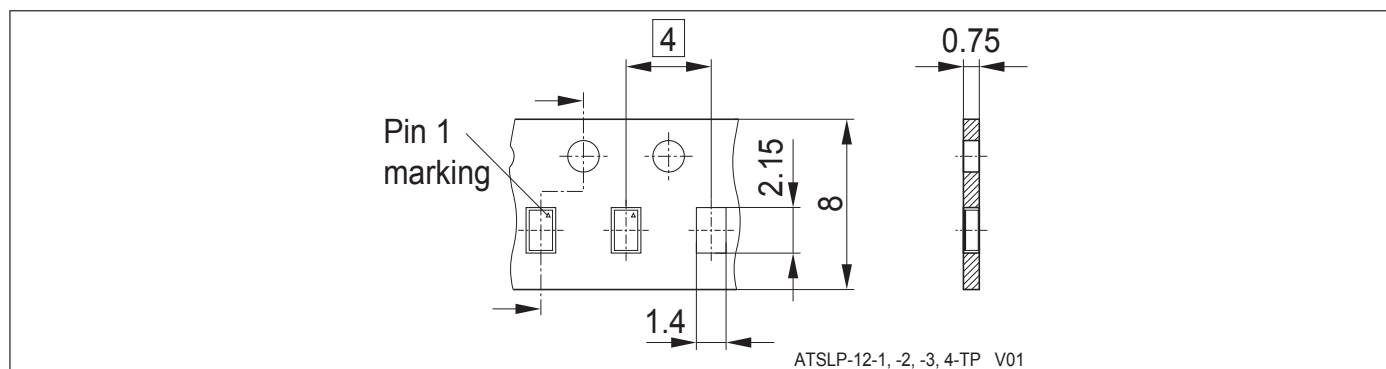
Figure 12: ATSLP-12-2 Carrier Tape
