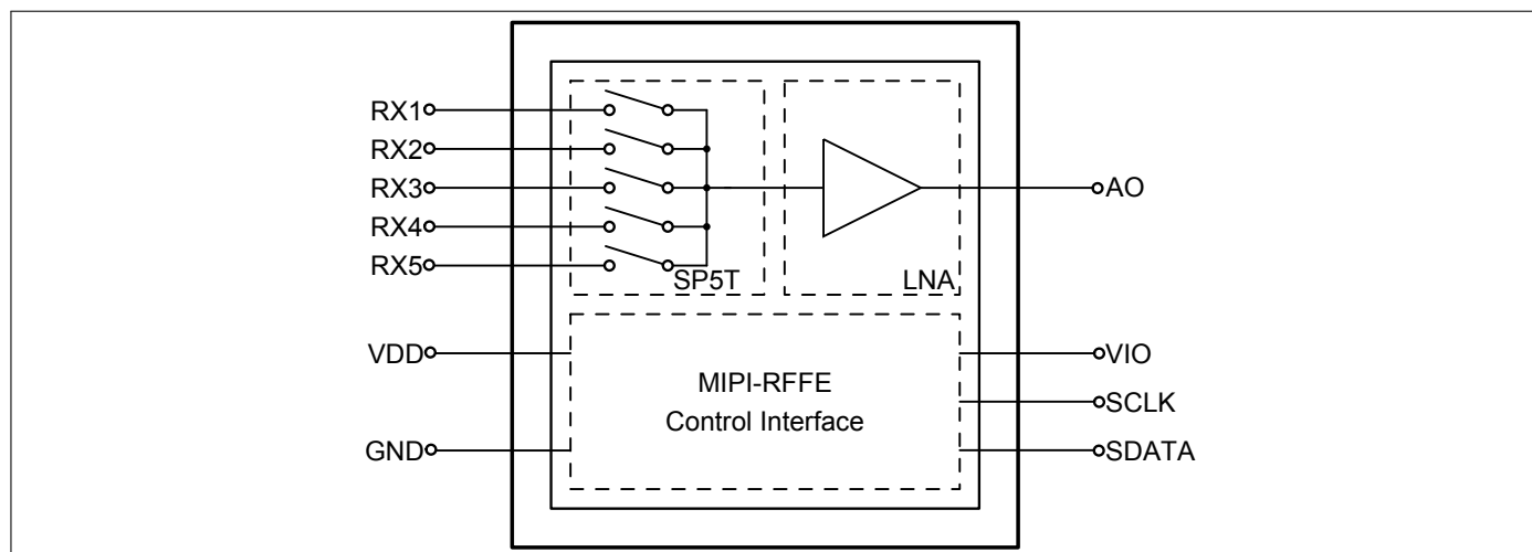
Figure 1: BGM15MA12 Block diagram
