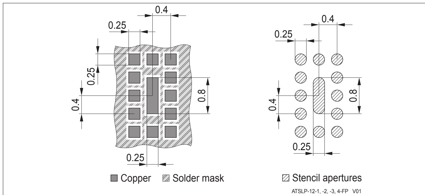
Figure 11: Footprint Recommendation
