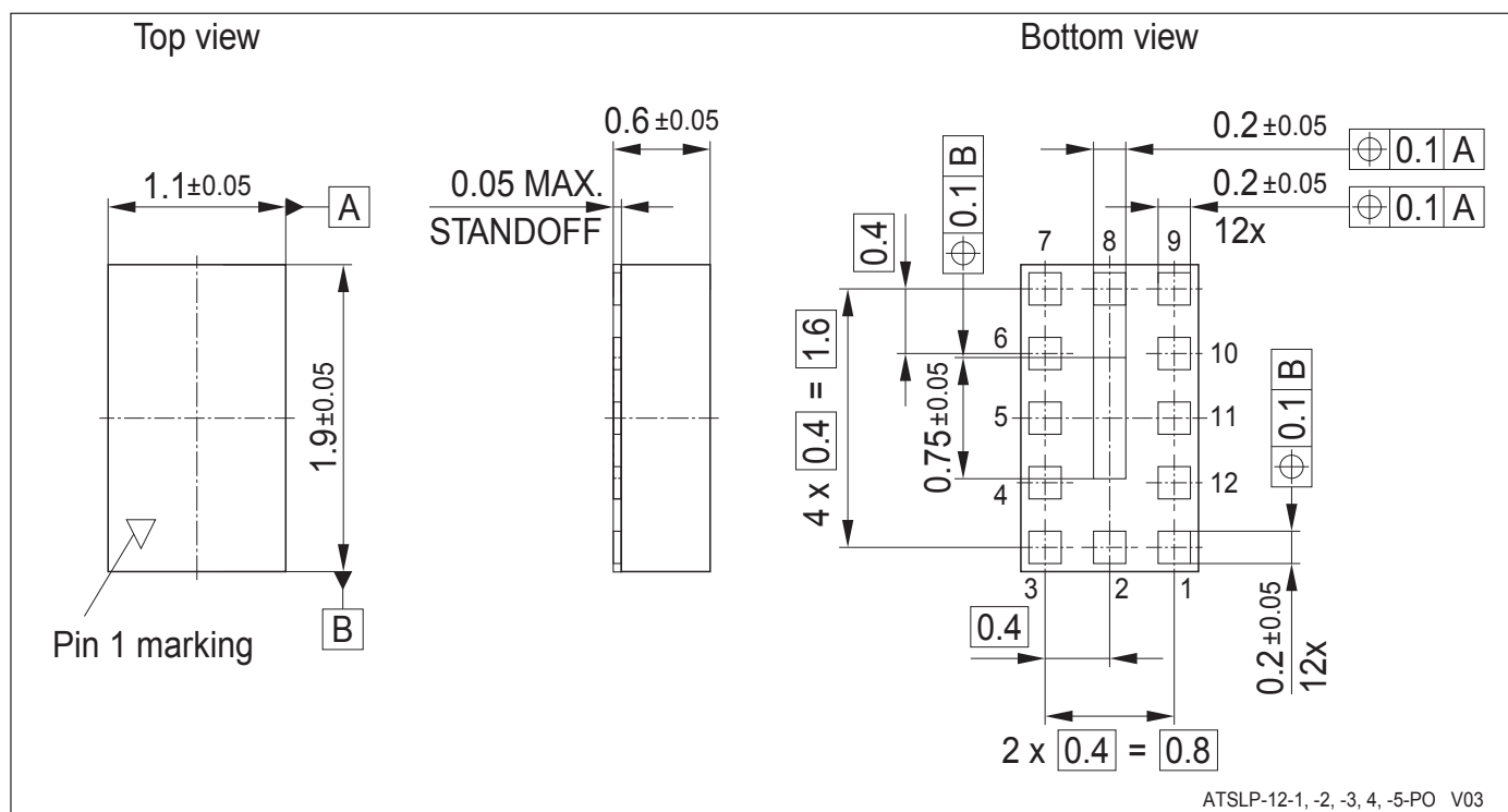
Figure 9: ATSLP-12-2 Package Outline (top, side and bottom views)
