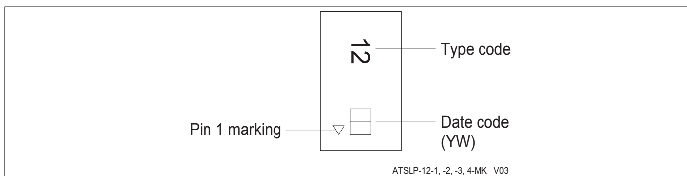
Figure 10: Marking Specification (top view)
