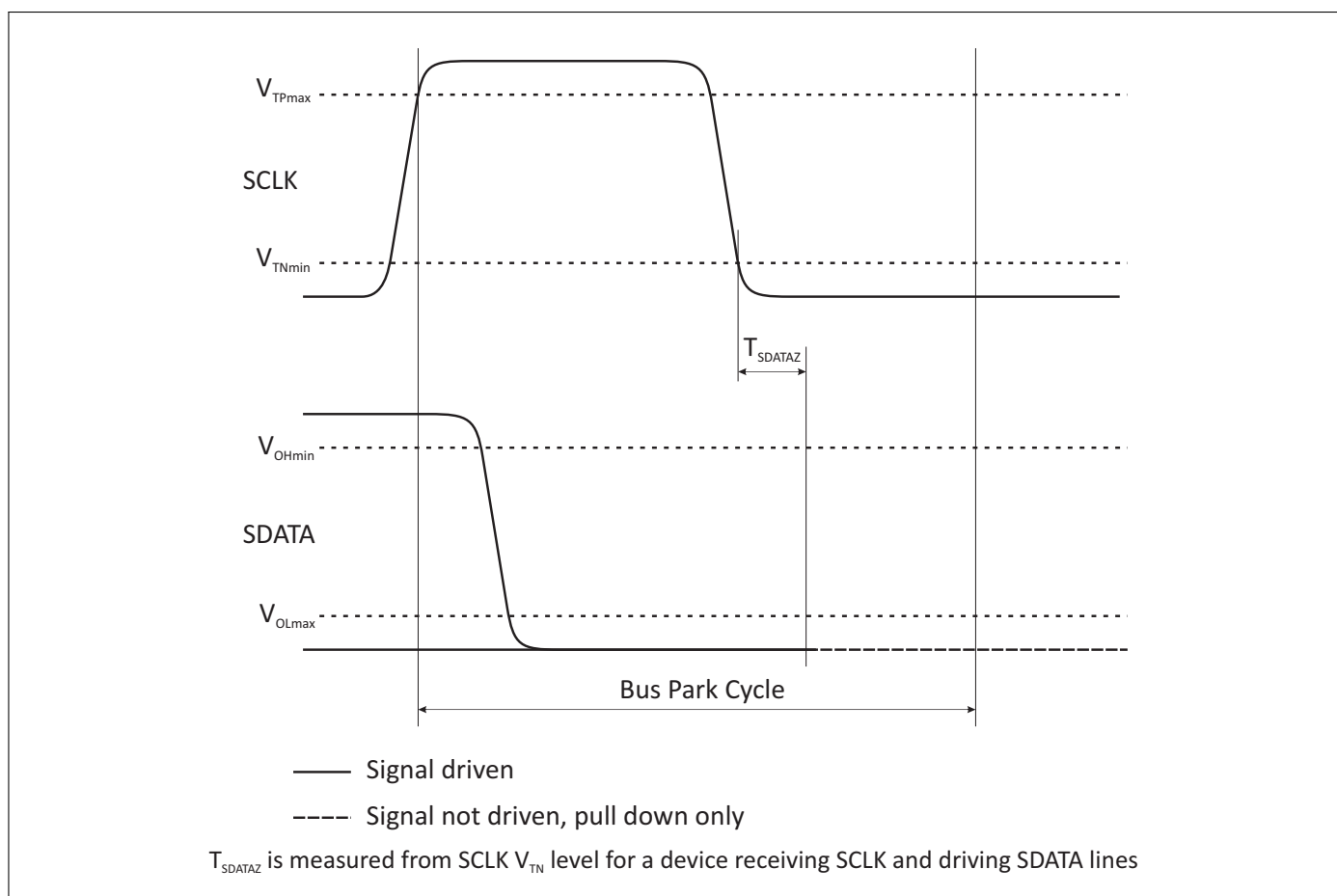
Figure 4: Bus park cycle timing
