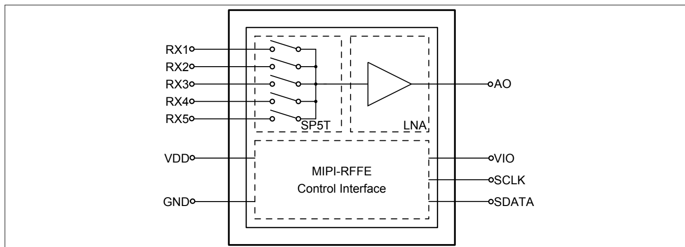
Figure 1: BGM15LA12 Block diagram
