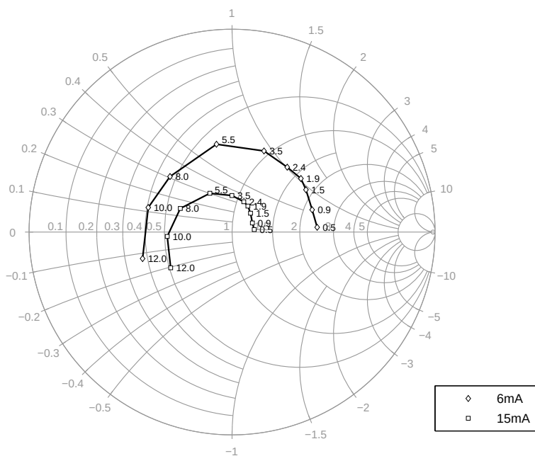
Figure 7-16 Source Impedance for Minimum Noise Figure Z_{opt} = f(f) , V_{CE} = 3\text{ V} , I_C = 6 / 15\text{ mA}
