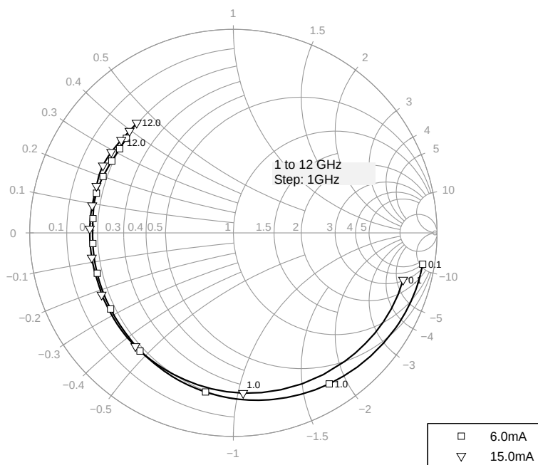
Figure 7-15 Input Matching S_{11} = f(f) , V_{CE} = 3\text{ V} , I_C = 6 / 15\text{ mA}
