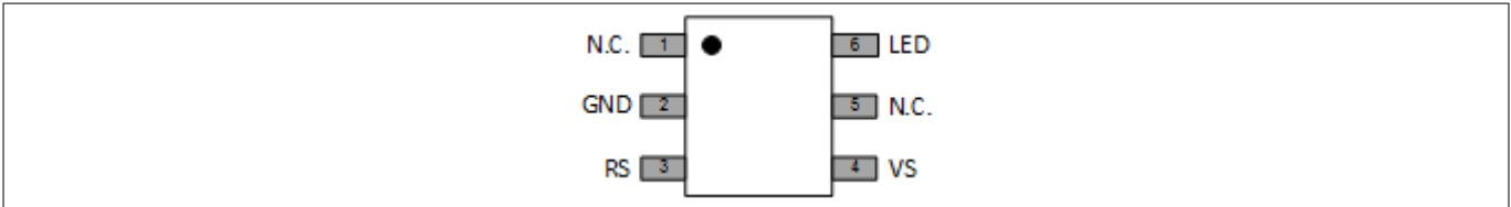
Figure 2 Pinout BCR430U
