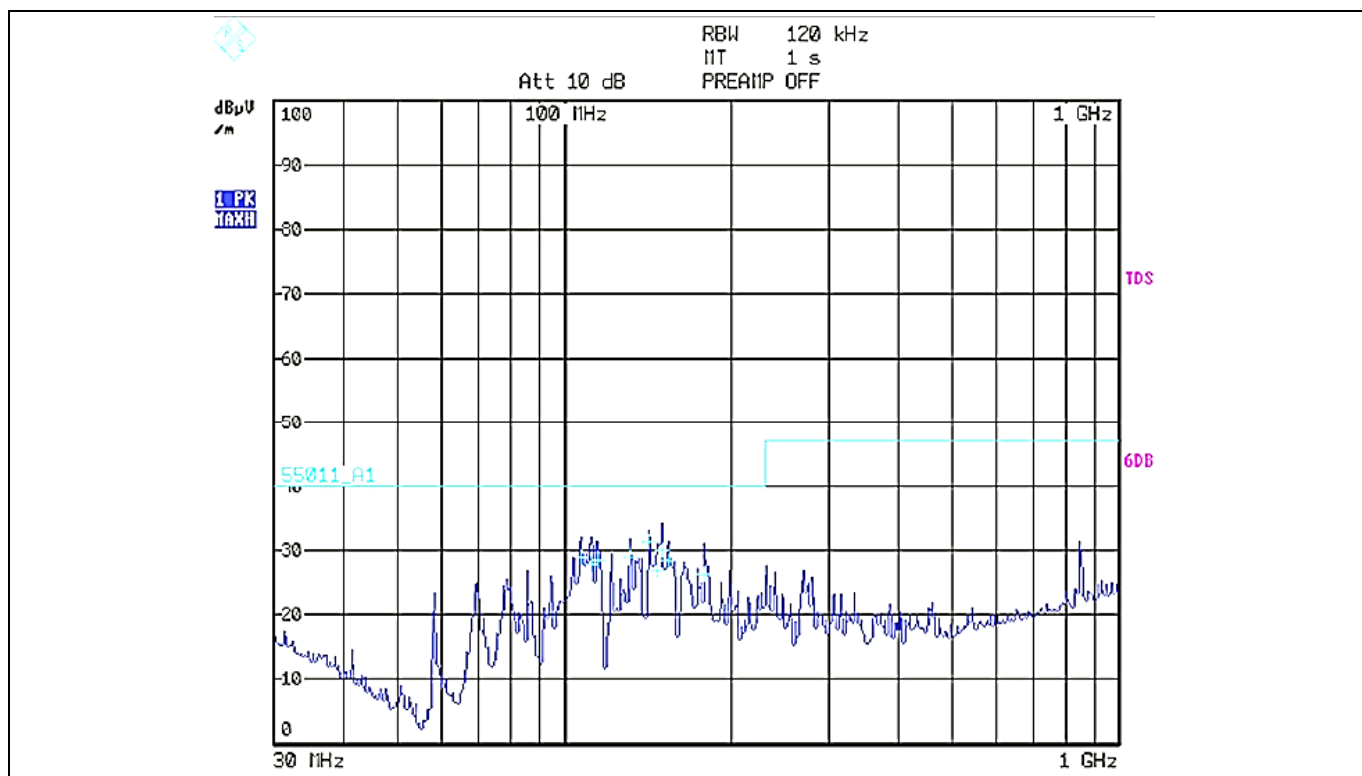
Figure 26 Radiated EMI according to EN55011, Group 1, Class A limits
