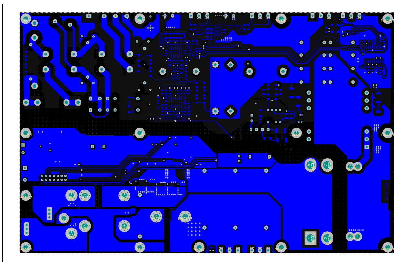
Figure 47 View of the power PCB bottom layer
