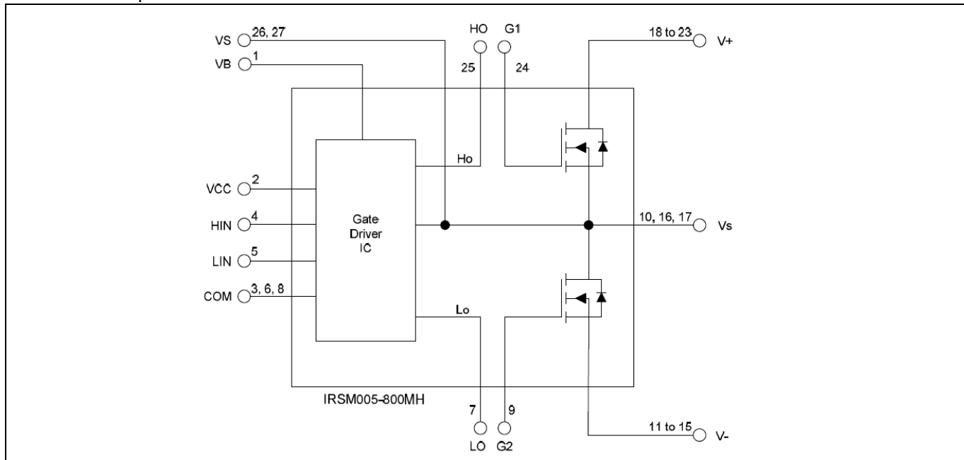
Figure 2 CIPOS™ Nano internal electrical schematic
