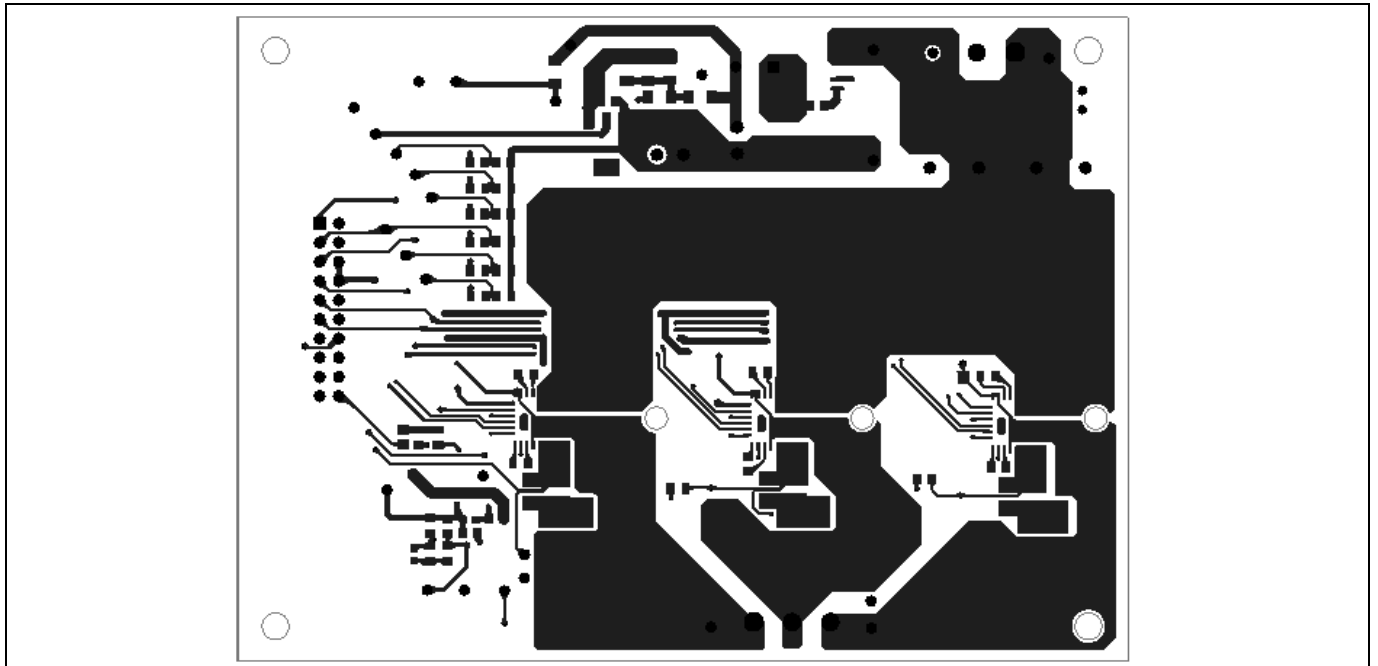
Figure 18 Top layer routing of the EVAL-M1-05F804 evaluation board
