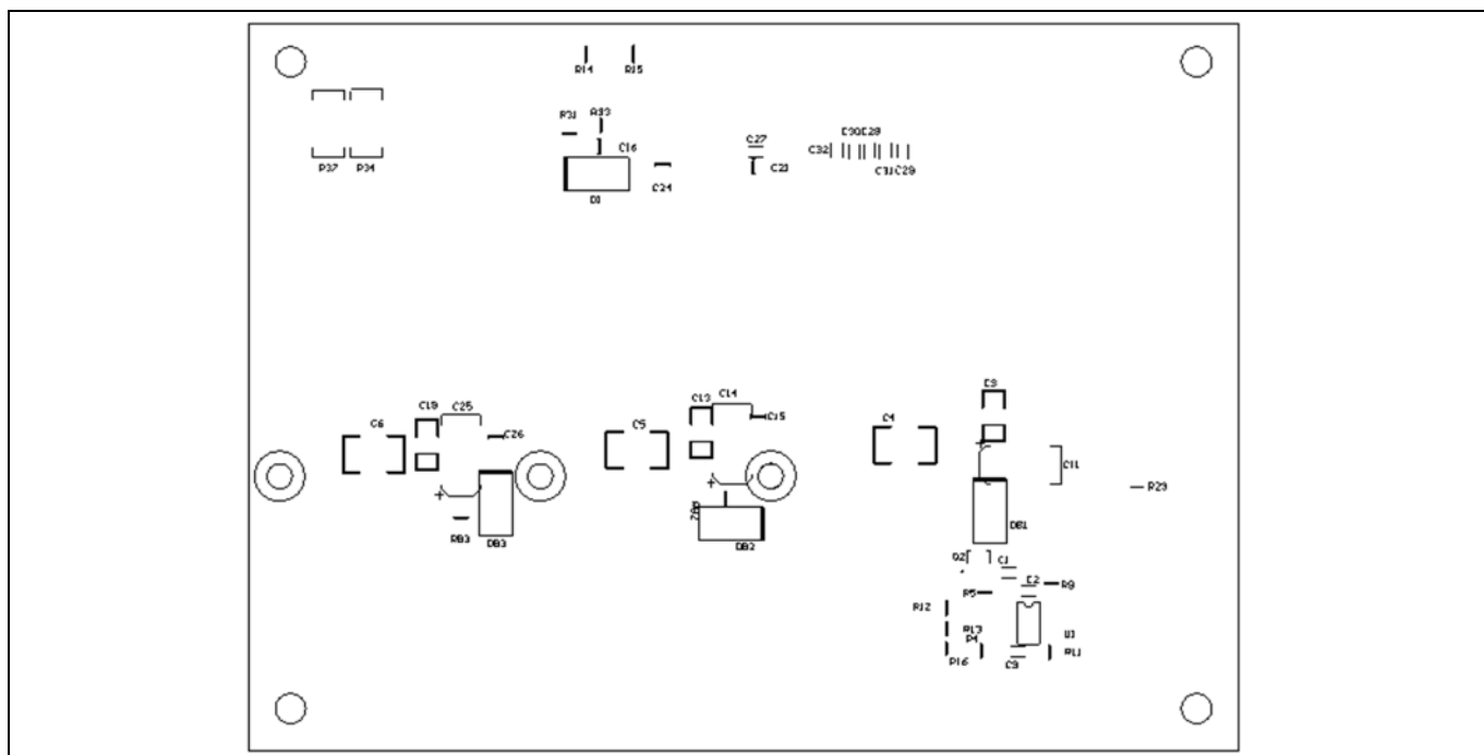
Figure 17 Bottom assembly print of the EVAL-M1-05F804 evaluation board
