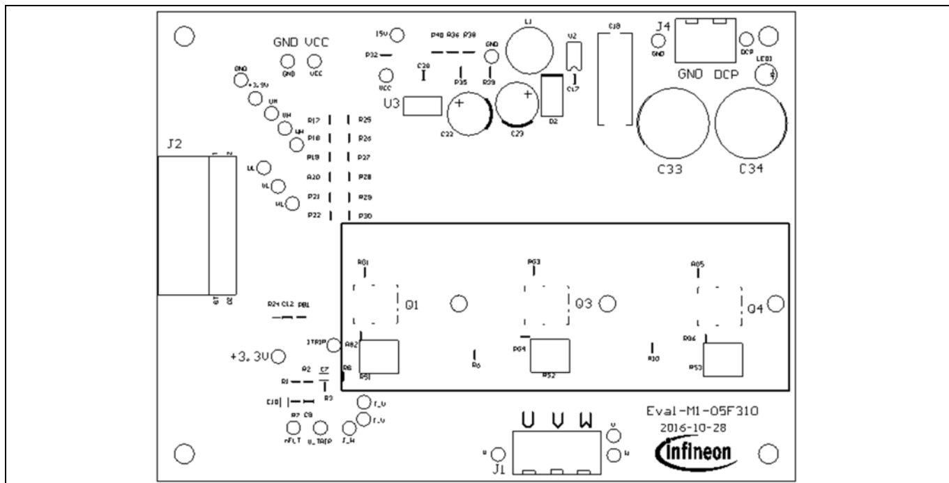
Figure 16 Top assembly print of the EVAL-M1-05F804 evaluation board
