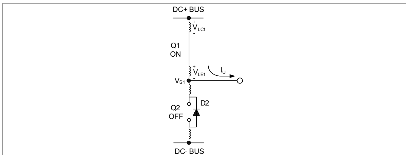
Figure 26 V_S positive
