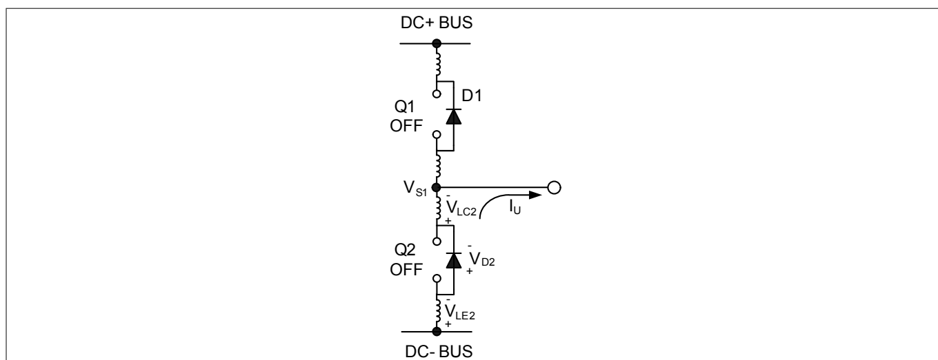
Figure 27 V_S negative
