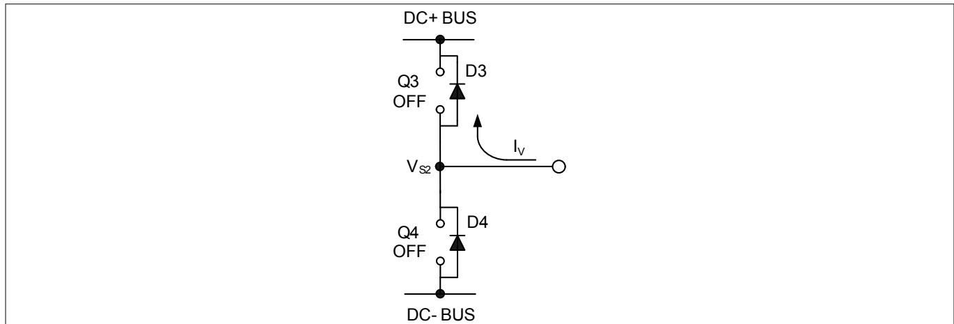
Figure 23 D3 conducting
