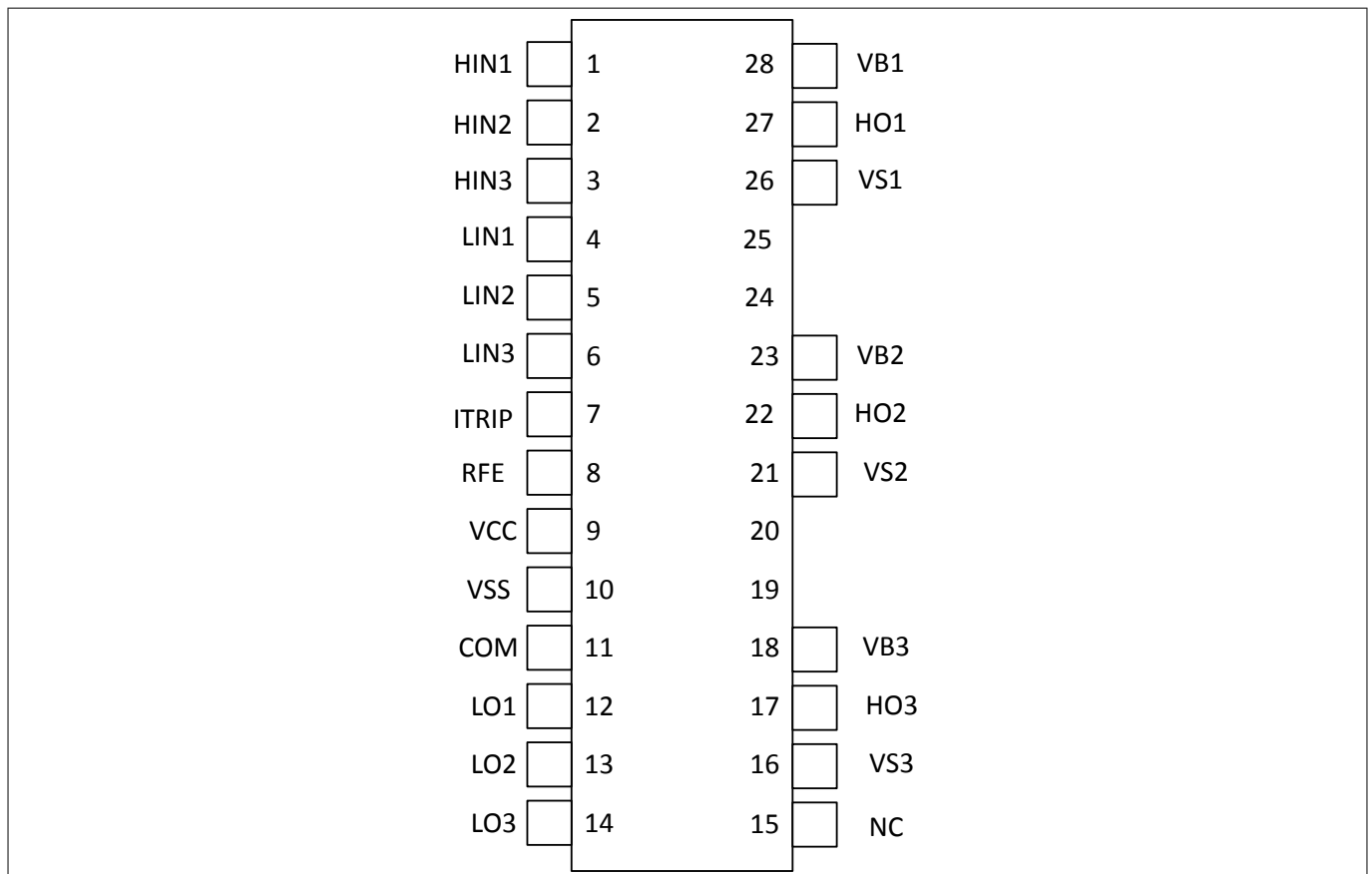
Figure 3 Lead Assignments
