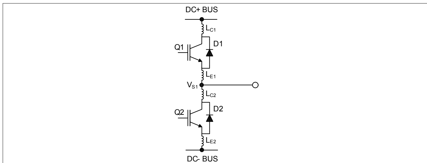
Figure 25 Parasitic elements
