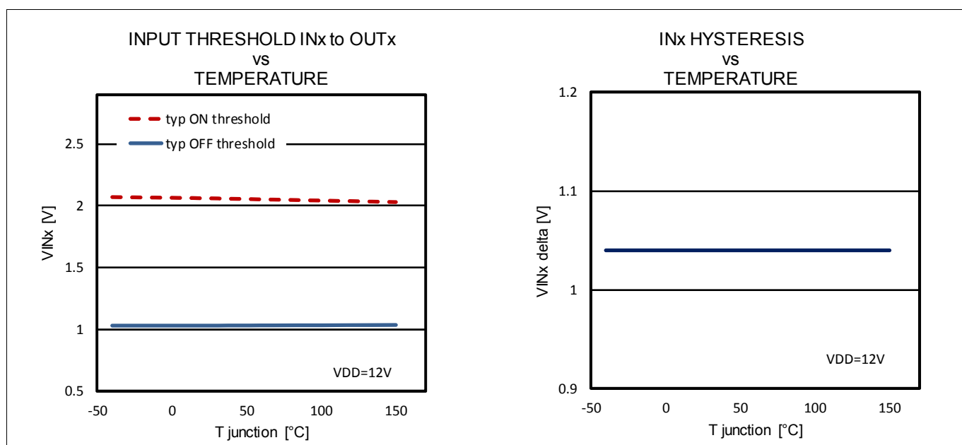
Figure 8 Input (INx) characteristic
