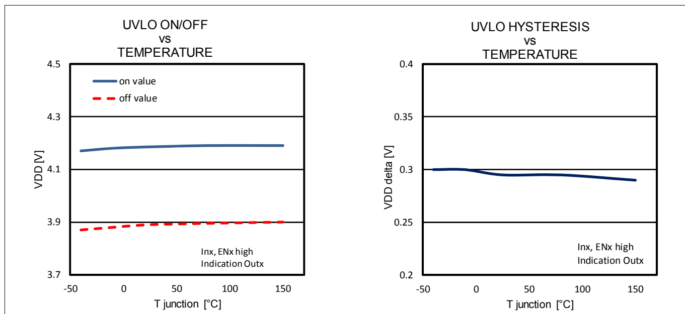
Figure 7 Undervoltage lockout (4.2V)
