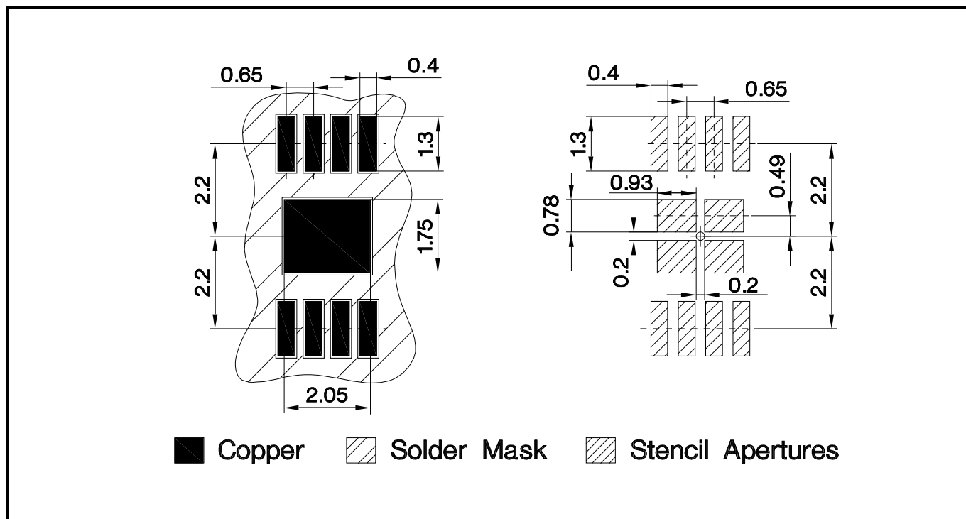
Figure 8-5 PG-TSSOP-8-1 footprint
