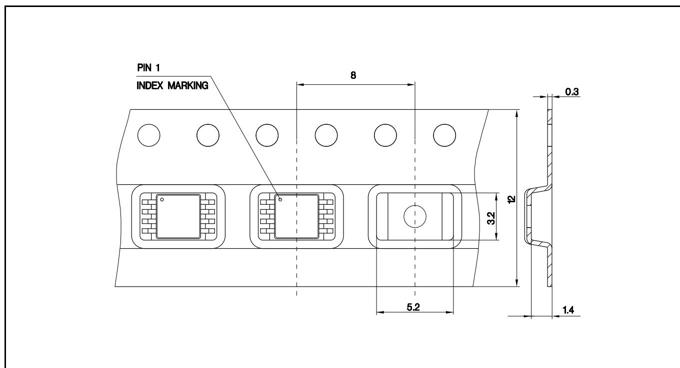
Figure 8-6 PG-TSSOP-8-1 packaging
