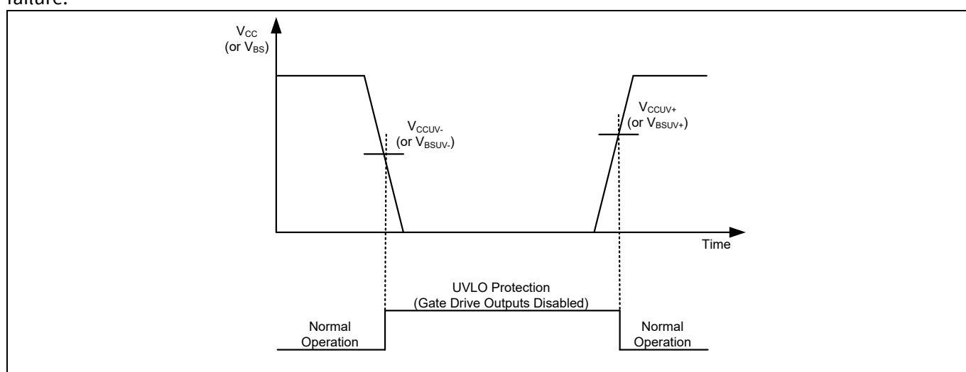
Figure 10 UVLO protection
