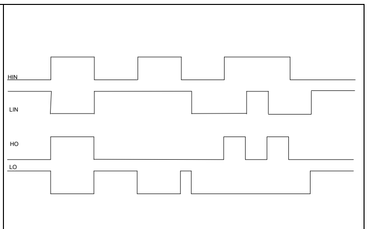
Figure 7 Input/output logic diagram
