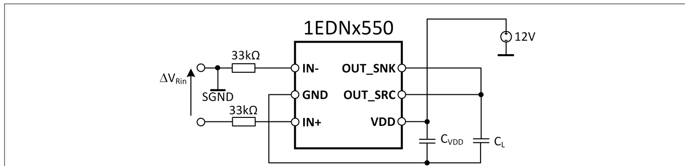
Figure 5 Test circuit
