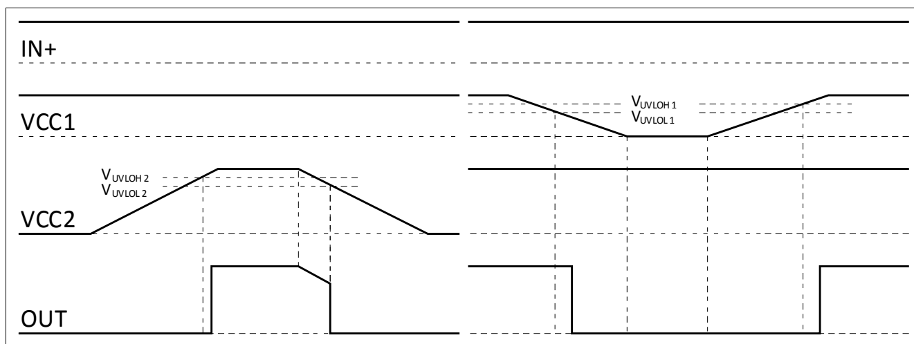
Figure 7 UVLO Behavior
