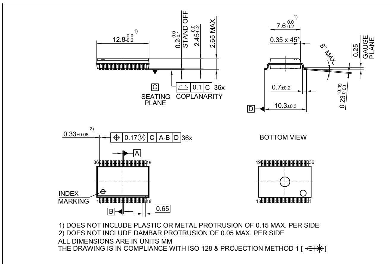
Figure 27 Package Dimensions
