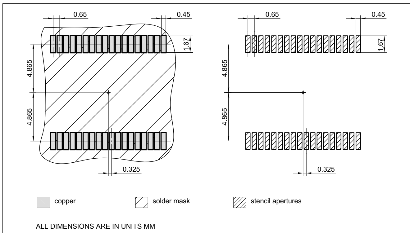
Figure 28 Recommended Footprint
