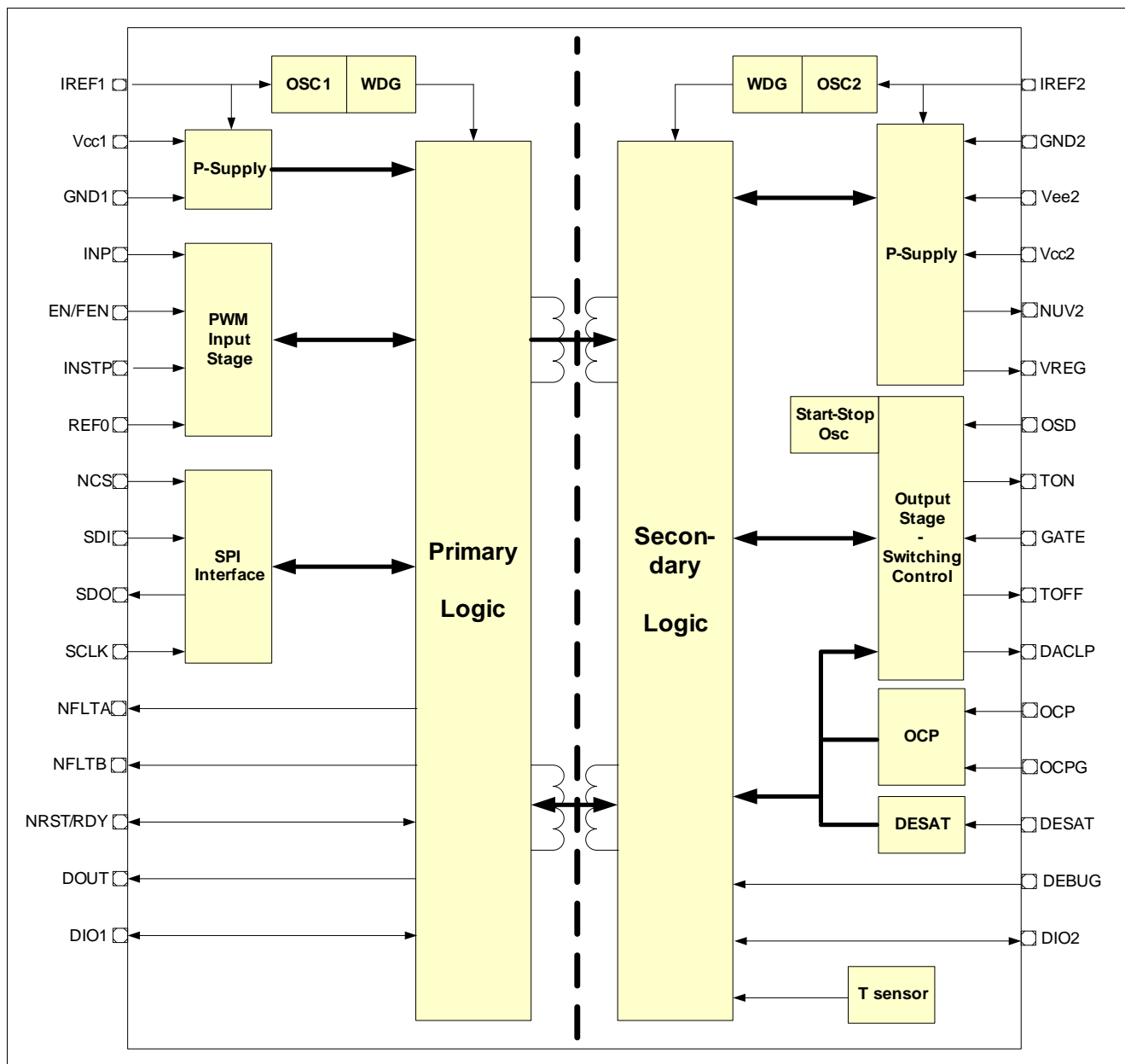
Figure 2-2 Block Diagram
