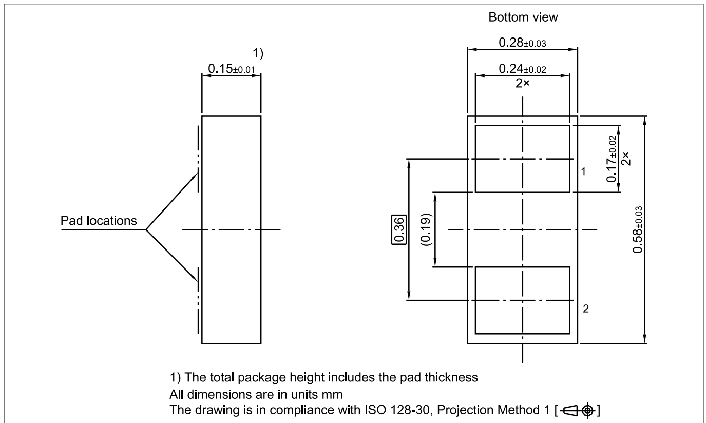
Figure 11 WLL-2-3 package
