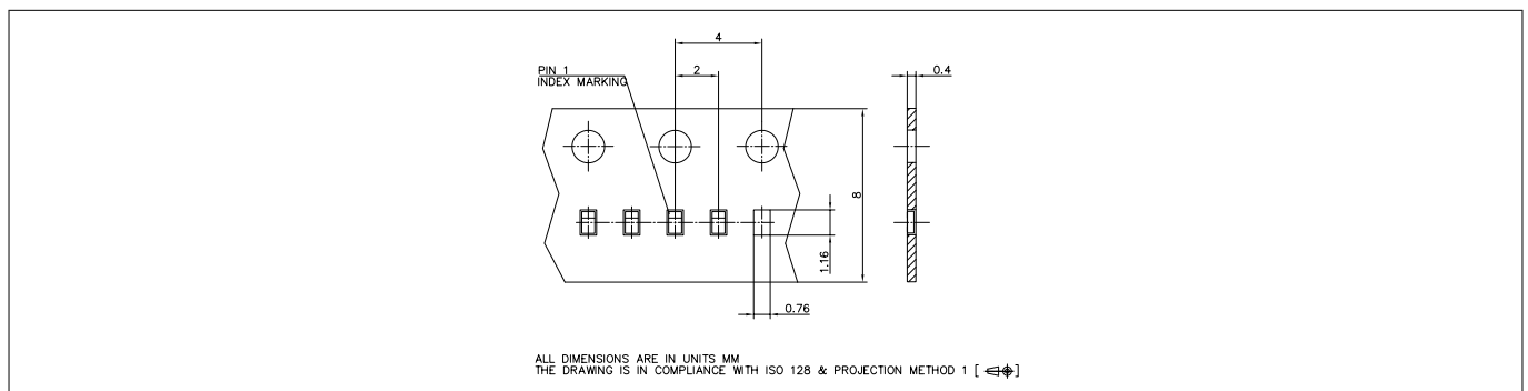
Figure 13 Tape dimensions
