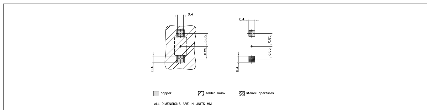
Figure 11 Foot print
