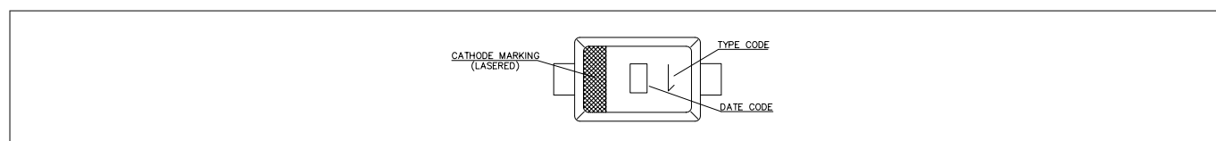
Figure 12 Marking layout
