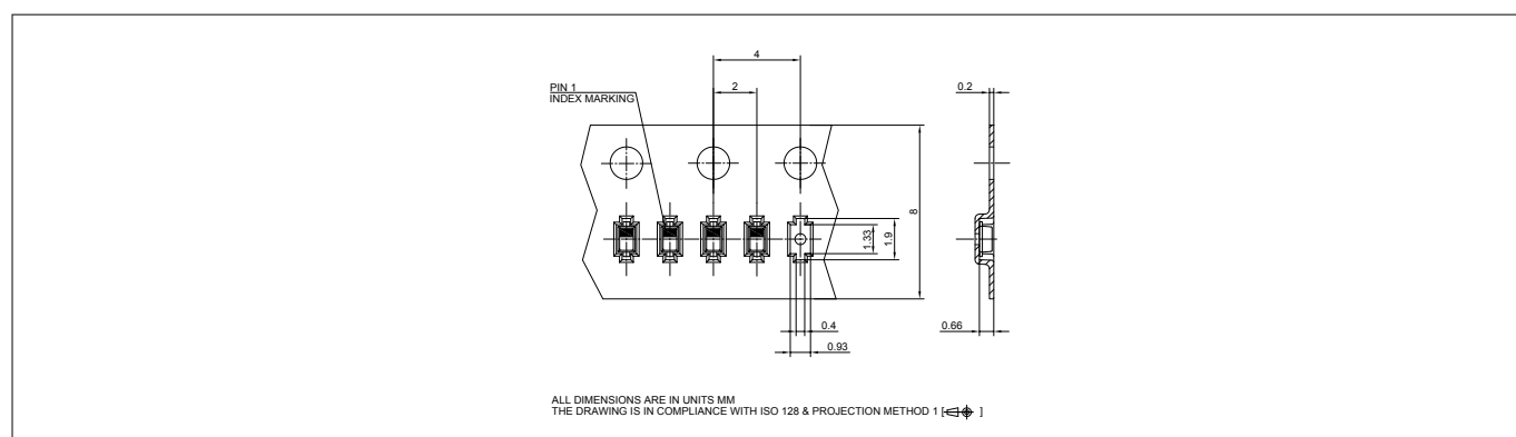
Figure 13 Tape dimensions
