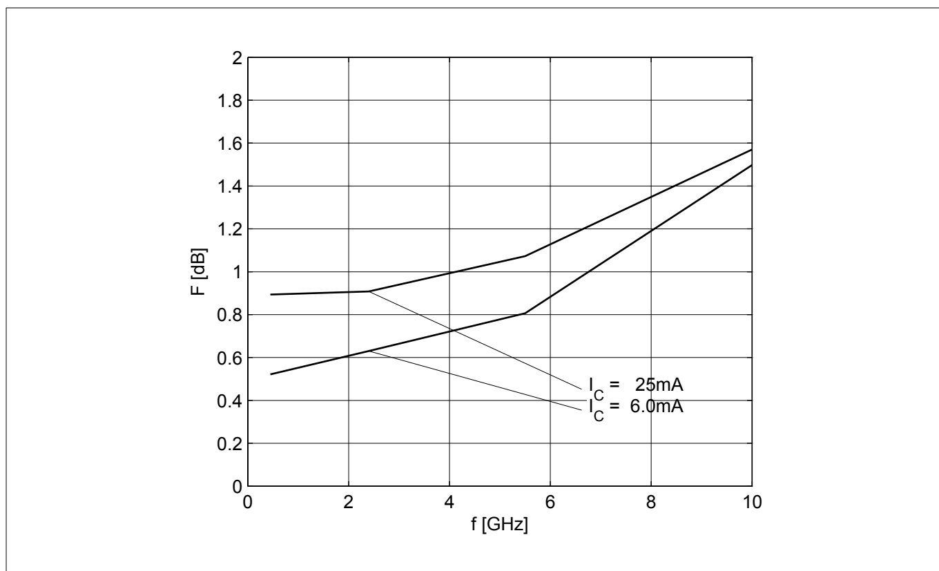
Figure 17 Noise figure NF_{\min} = f(f) , V_{CE} = 3\text{ V} , Z_S = Z_{S,\text{opt}} , I_C = 6 / 25\text{ mA}
