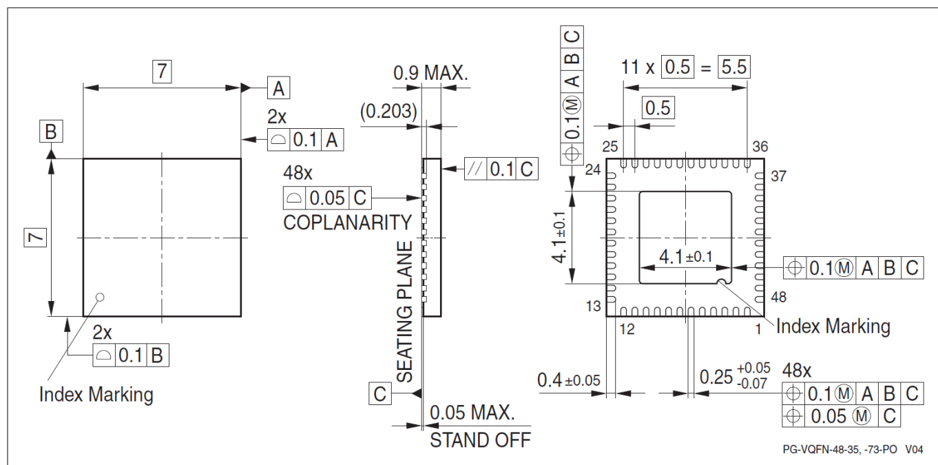
Figure 21 PG-VQFN-48-73
