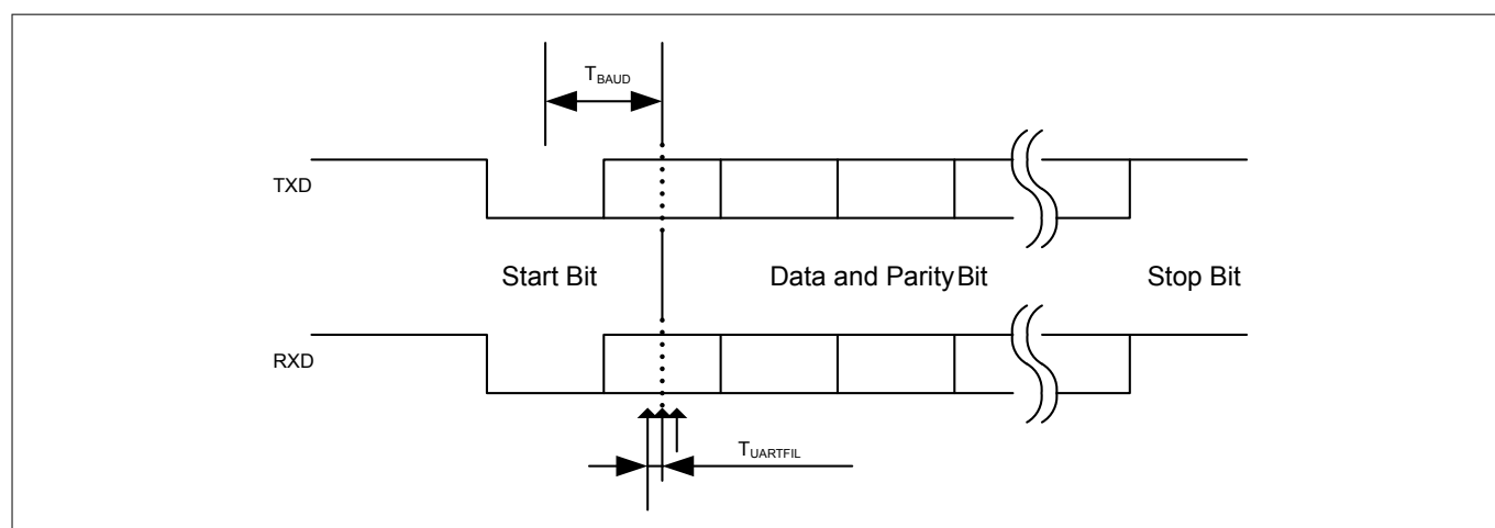
Figure 16 UART timing
