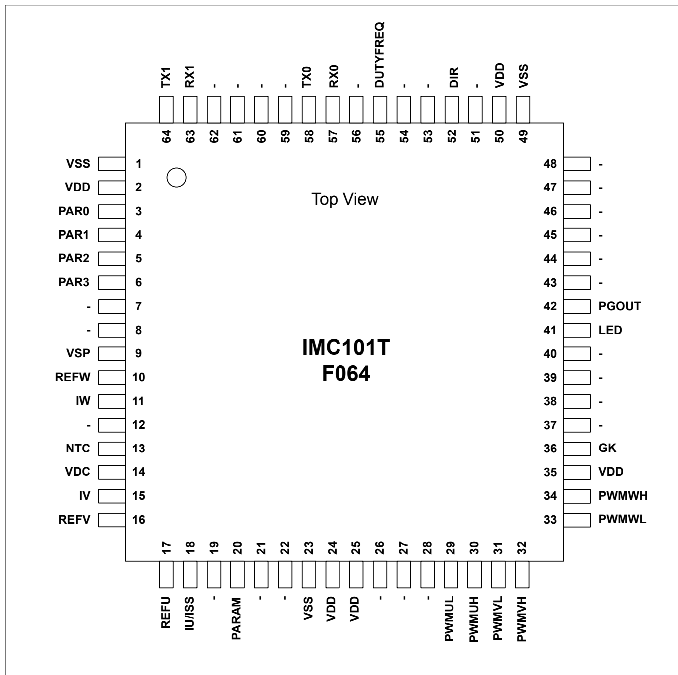
Figure 4 IMC101T-F064
