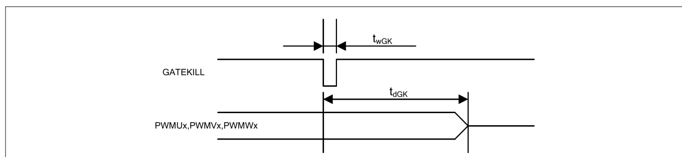
Figure 15 Fault timing
