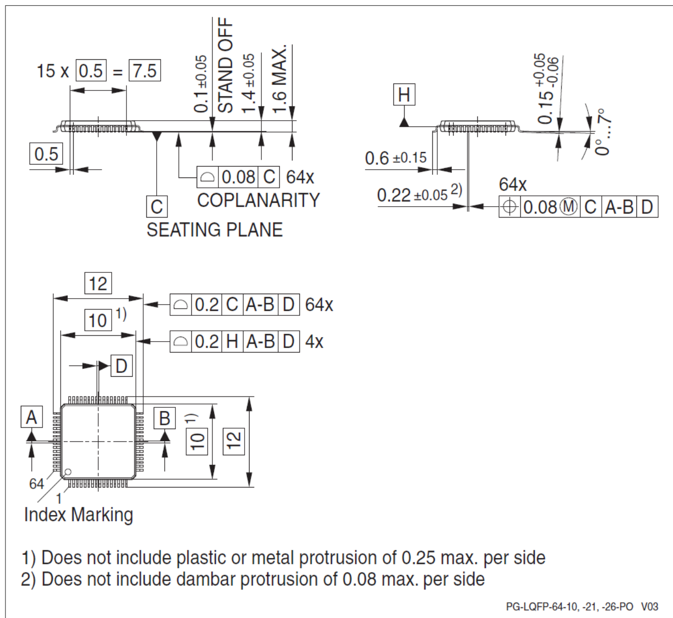
Figure 23 PG-LQFP-64-26
