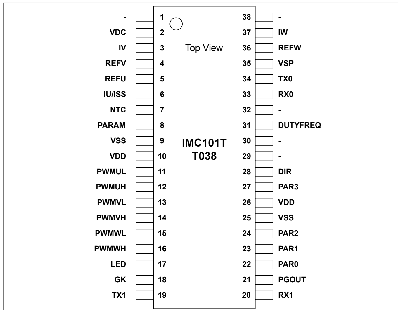
Figure 2 IMC101T-T038
