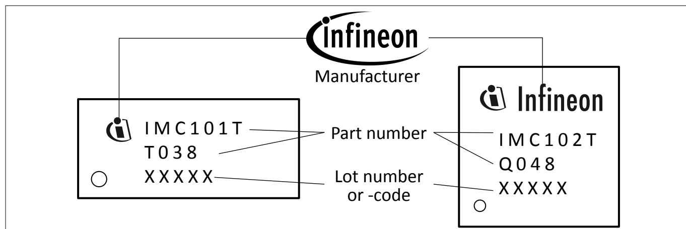
Figure 24 Part marking
