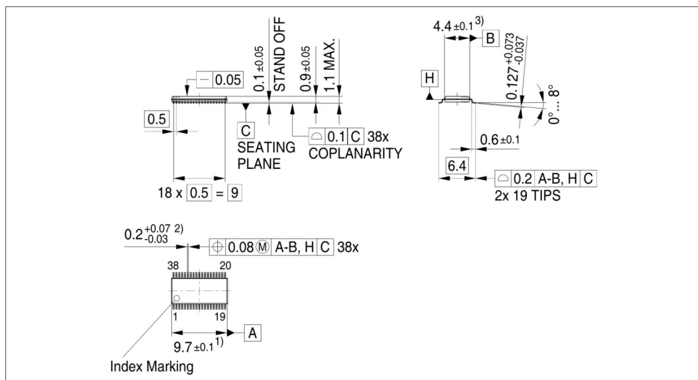
Figure 20 PG-TSSOP-38-9
