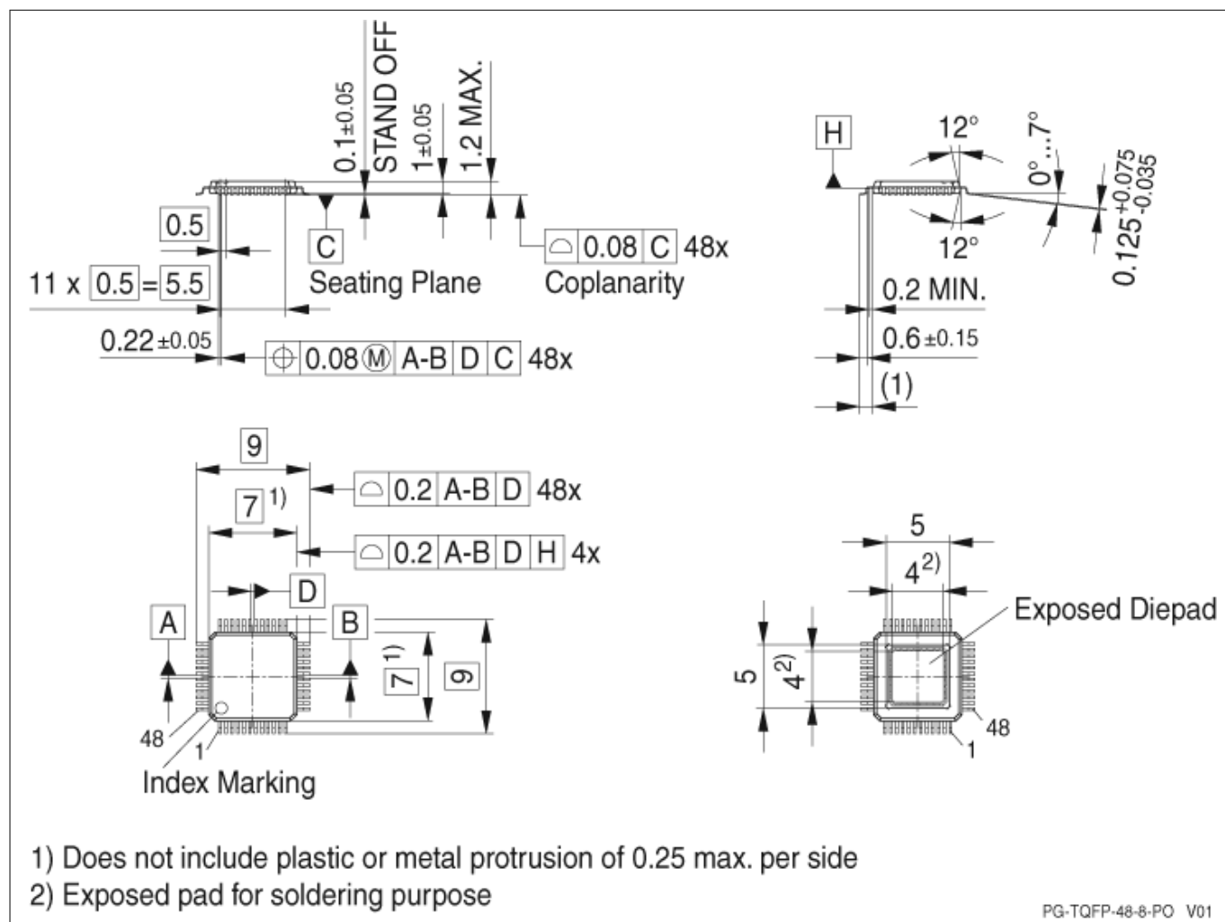
Figure 22 PG-TQFP-48
