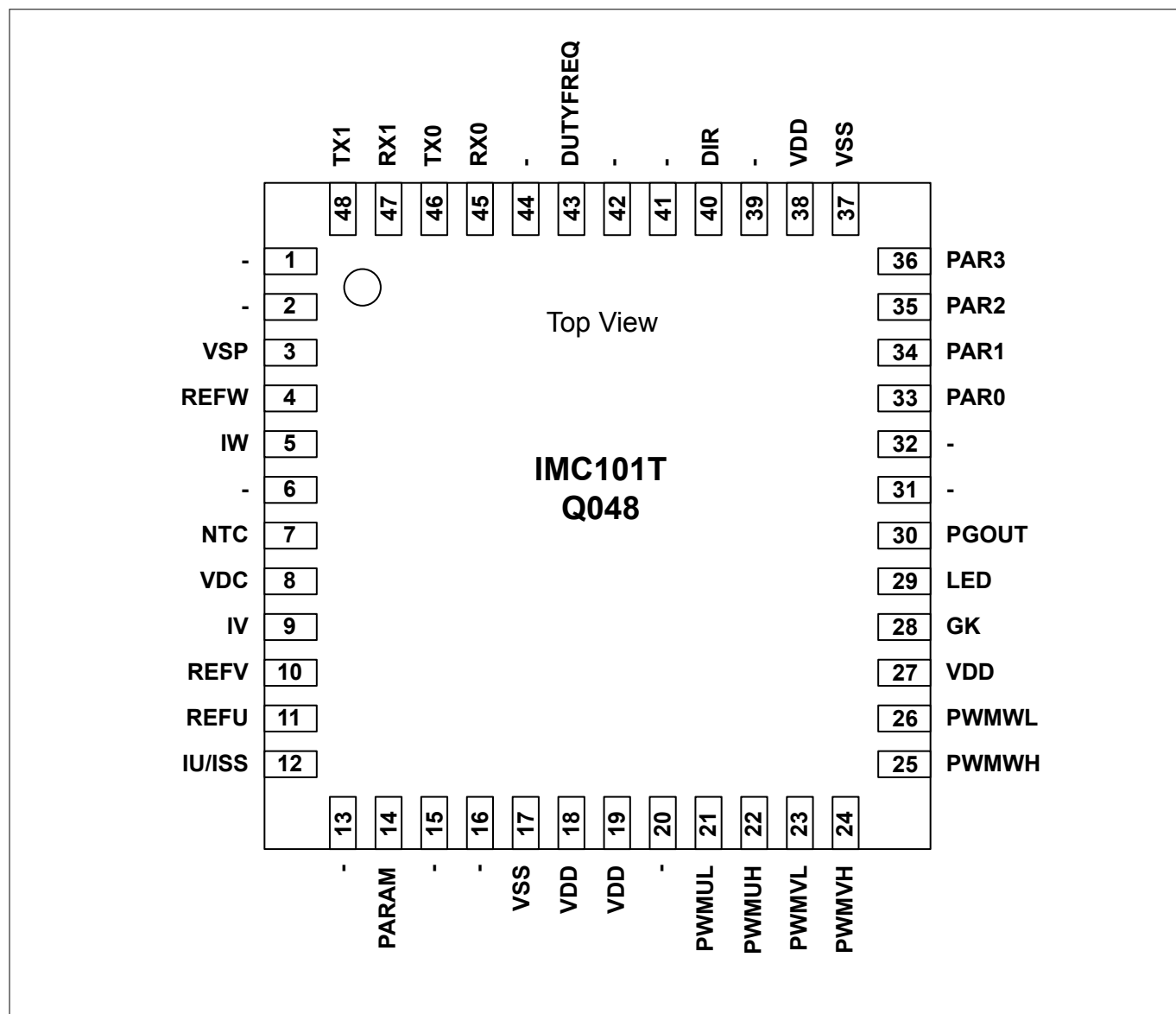
Figure 3 IMC101T-Q048
