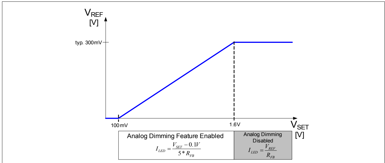
Figure 16 Voltage V_{SET} versus LED current
