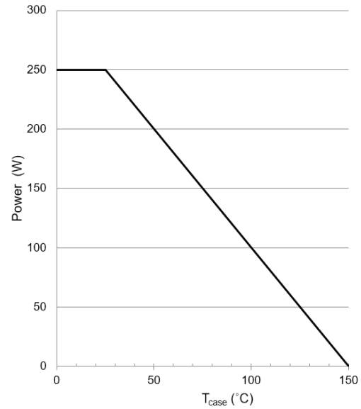
Figure 14: Power Derating vs. T_{case}
