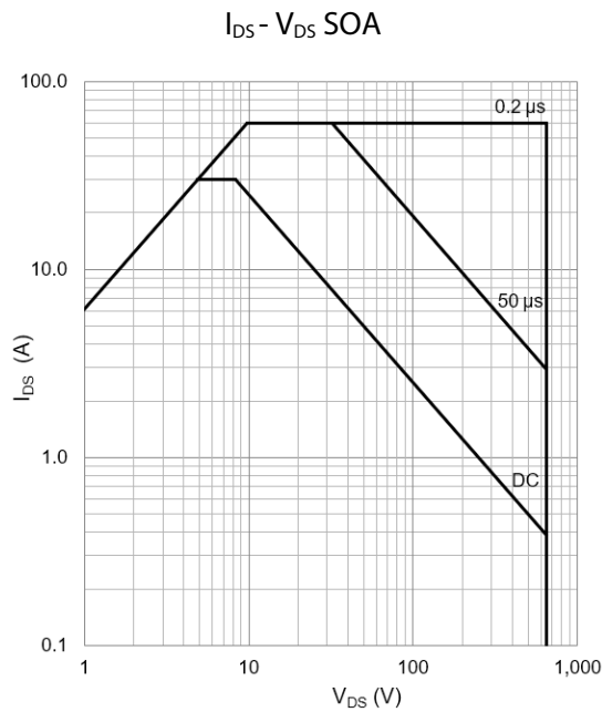
Figure 13: Safe Operating Area @ T_{case} = 25^\circ C
