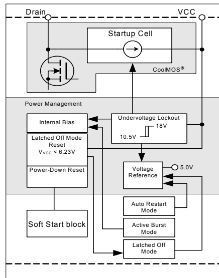
Figure 3 Power Management
