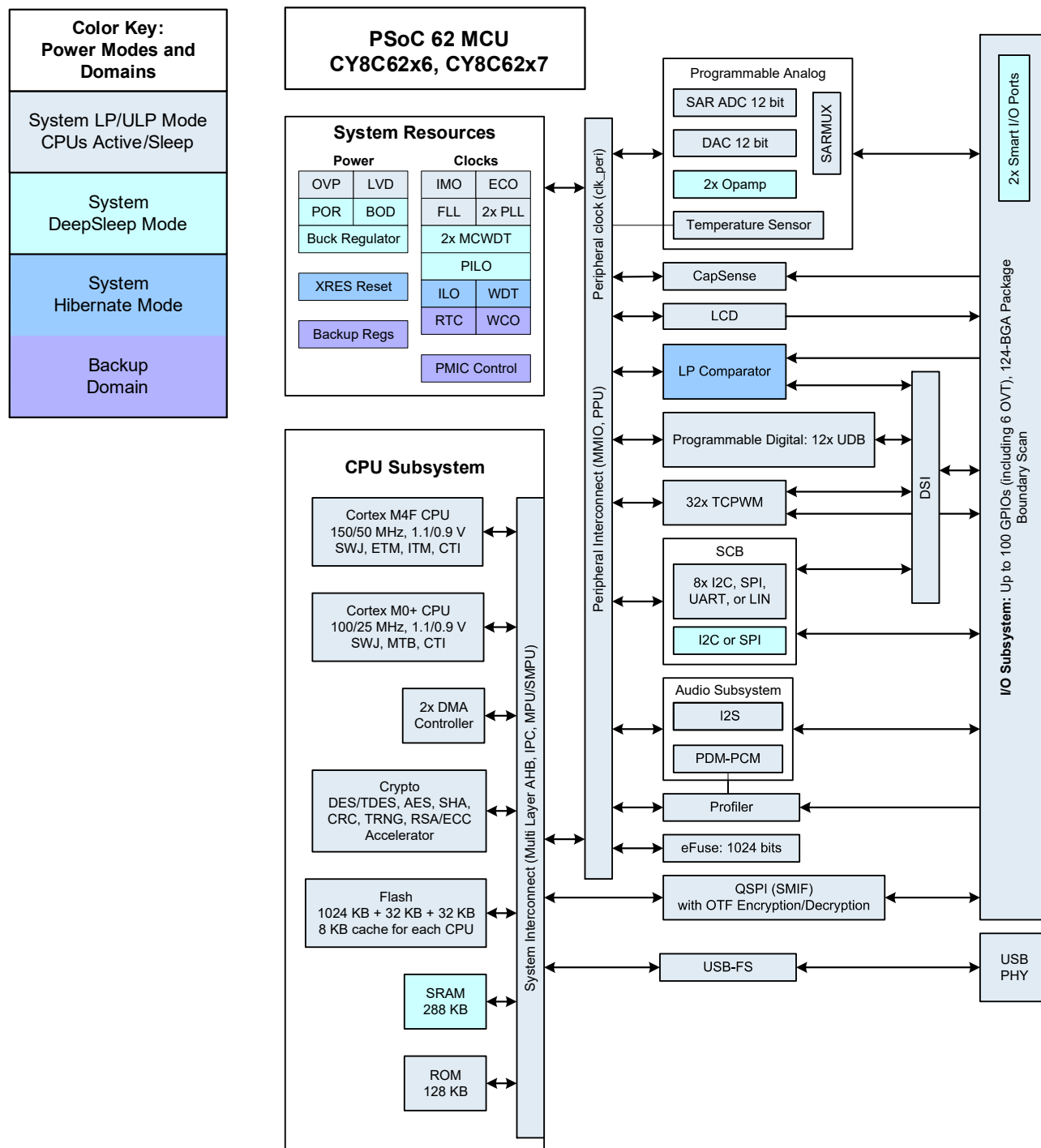
Figure 3. Block Diagram
