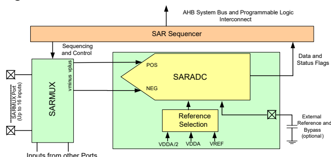
Figure 5. SAR ADC
