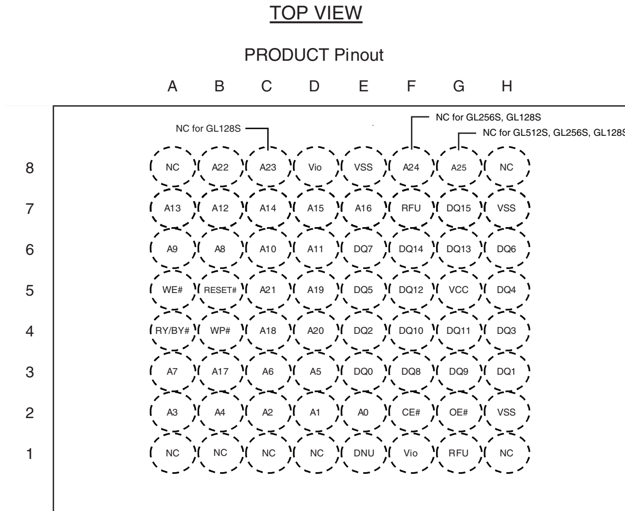
Figure 35. 64-ball Fortified Ball Grid Array [83], [84], [85]
