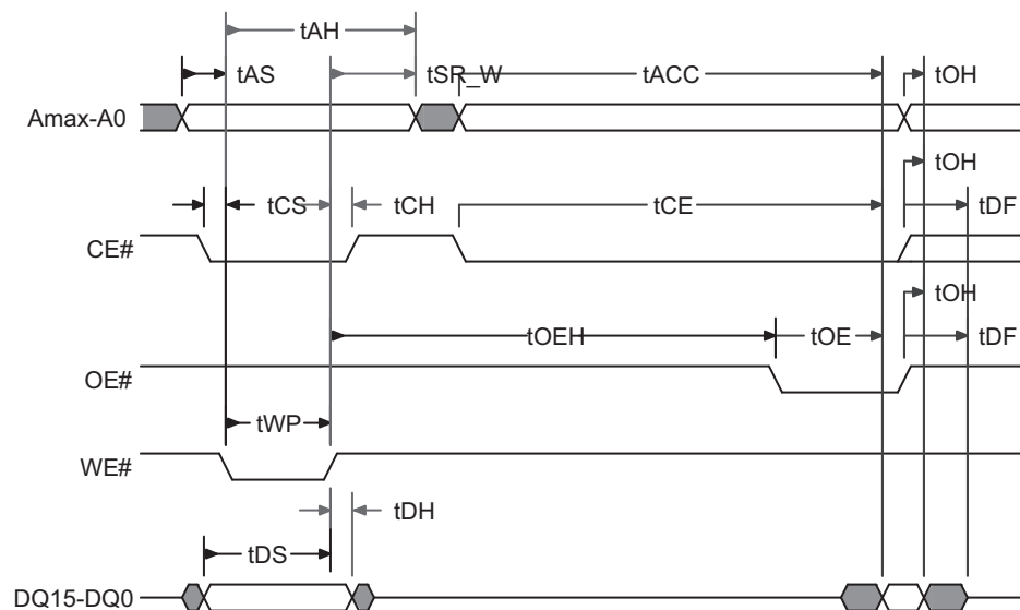
Figure 23. Write to Read ( t_{CE} ) Operation Timing Diagram
