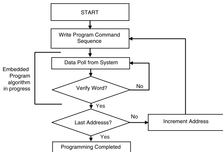
Figure 3. Word Program Operation
