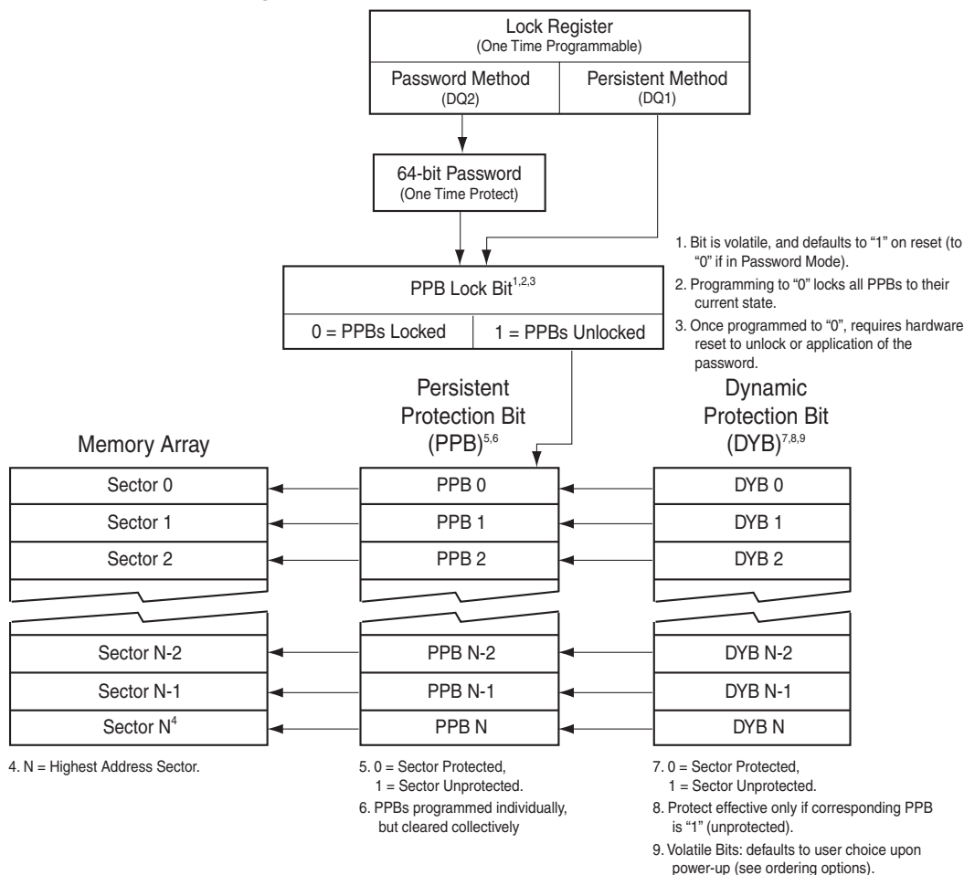
Figure 2. Advanced Sector Protection Overview
