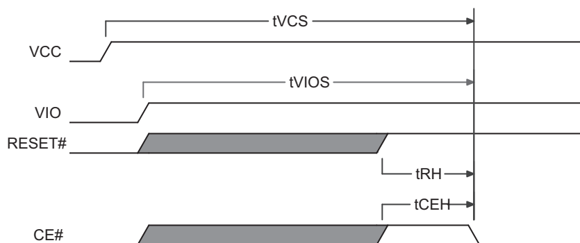
Figure 15. Power-Up Diagram
