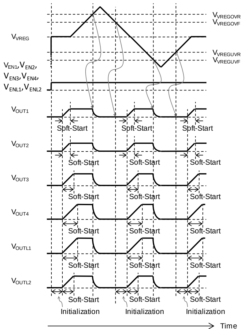
Figure 10-15 VREG OVLO/UVLO Timing Chart
