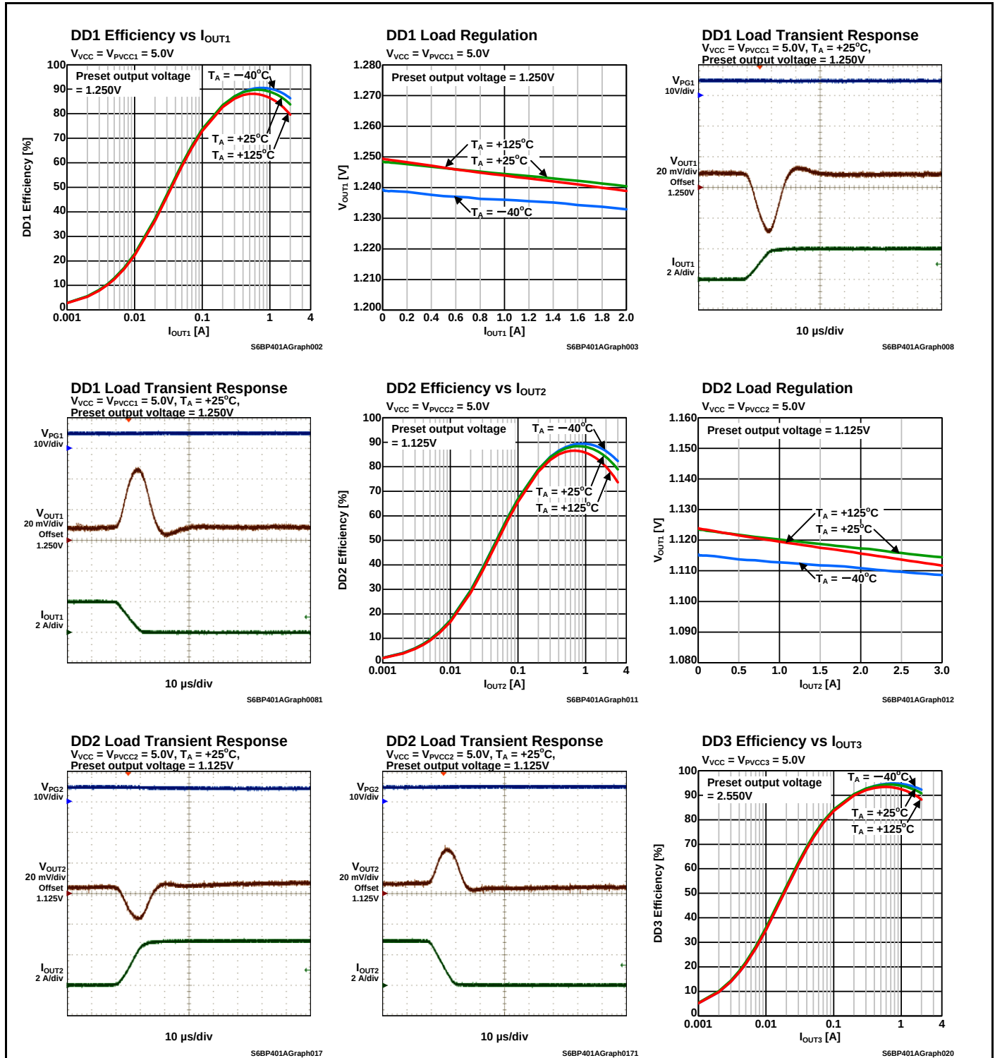
Figure 12-1 DC/DC Converter
