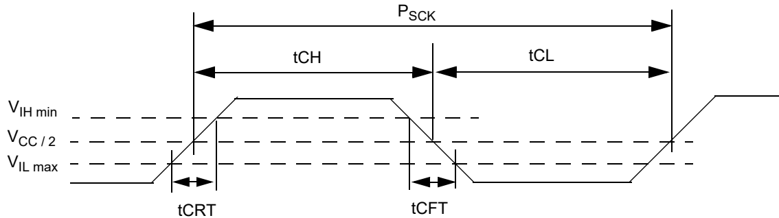
Figure 28. Clock Timing
