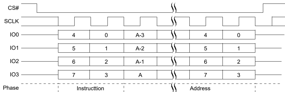
Figure 76. Parameter Sector Erase (P4E 20h or 4P4E 21h) QPI Mode Command Sequence [53]
