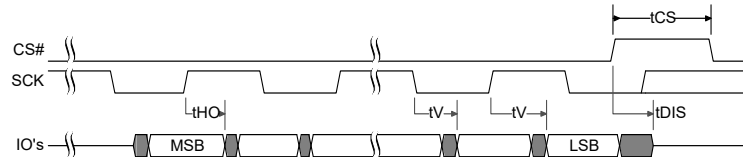
Figure 34. SPI DDR Output Timing
