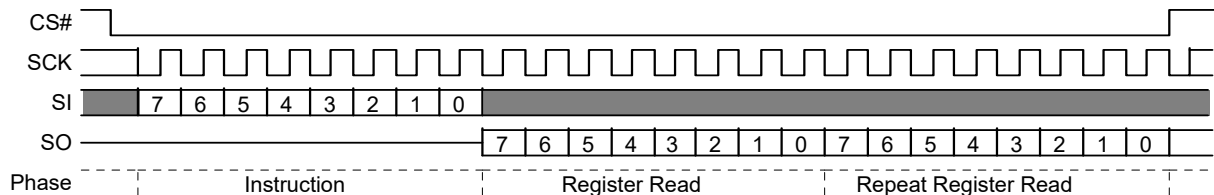
Figure 56. DLP Read (DLPRD) Command Sequence
