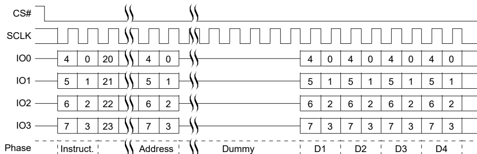
Figure 59. Read Any Register, QPI Mode, CR2[7] = 0, Command Sequence
