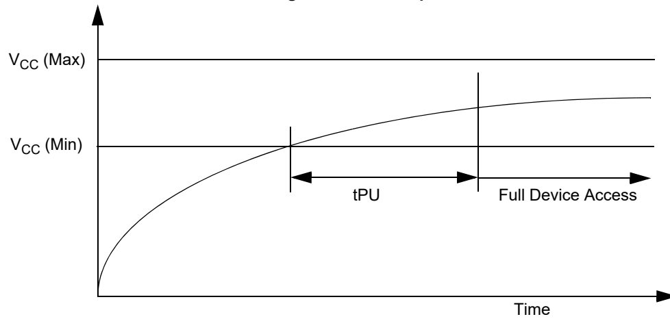
Figure 18. Power-up
