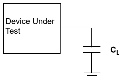
Figure 21. Test Setup
