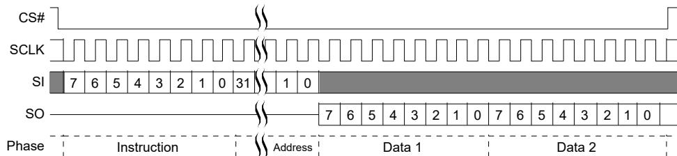
Figure 9. Single Bit Wide I/O Command without latency
