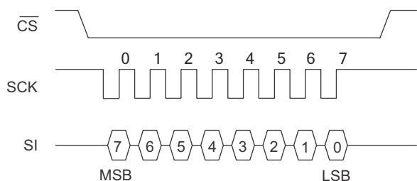
Figure 6. SPI Mode 3
