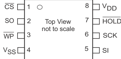
Figure 2. 8-pin DFN pinout
