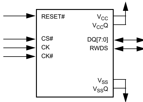
Figure 5. HyperRAM Interface [3]
