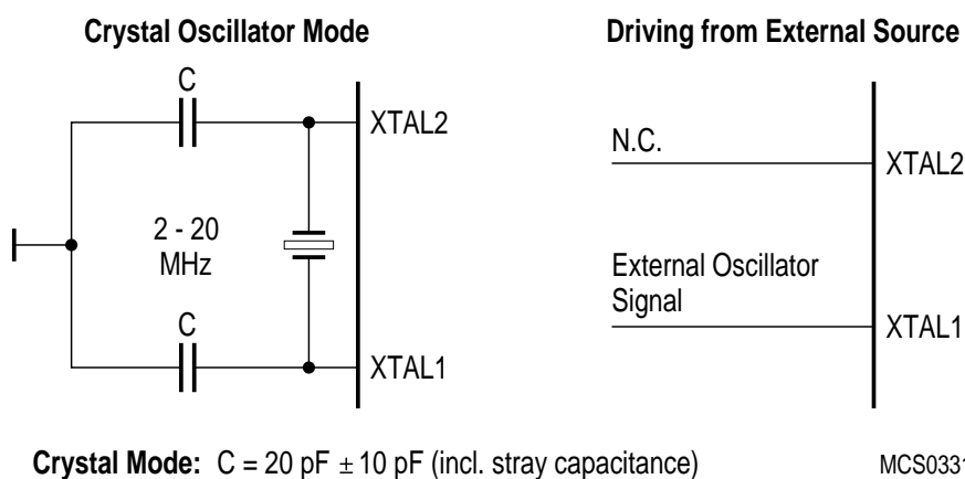
Figure 44 Recommended Oscillator Circuits for Crystal Oscillator
