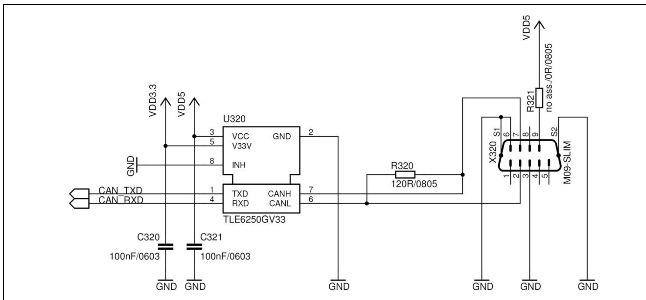
Figure 4 CAN Interface
