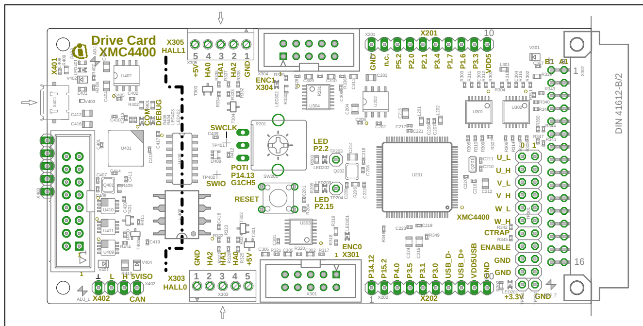
Figure 21 Component Placement
