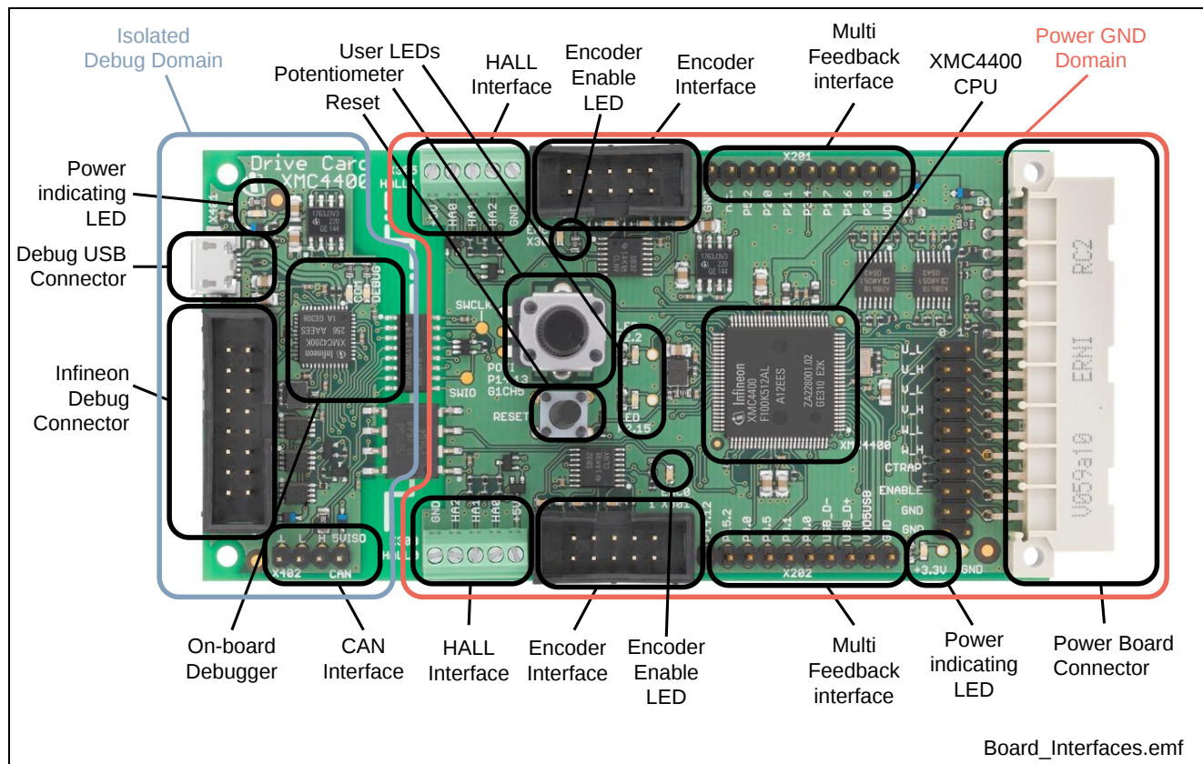
Figure 2 XMC4400 Drive Card (KIT_XMC4400_DC_V1)
