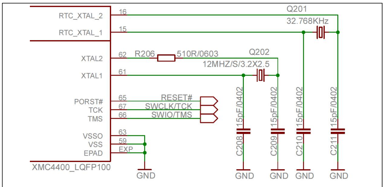
Figure 6 Clock Generation
