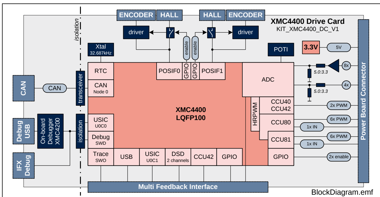
Figure 1 Block Diagram of KIT_XMC4400_DC_V1
