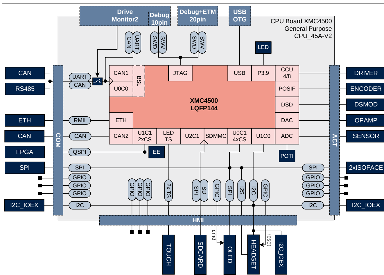
Figure 1 CPU_45A-V2 Board Block Diagram
