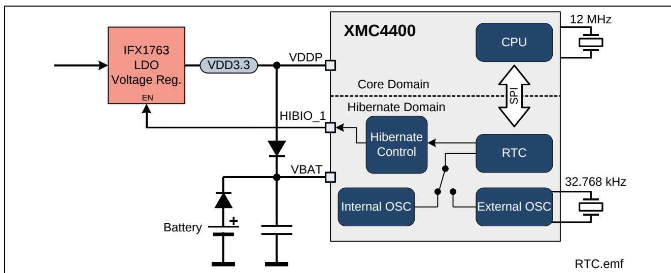
Figure 19 XMC4400 Power Domains and Real Time Clock
